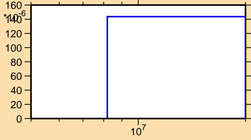
\sigma vs. E for ^{180}\text{Lu}(n,d)
