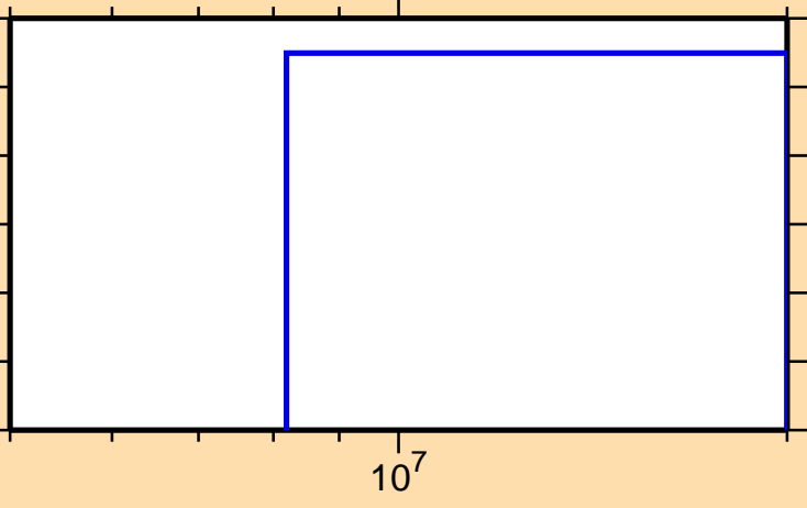
\sigma vs. E for ^{180}\text{Lu}(n,2n\alpha)
