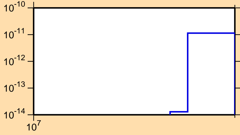
\sigma vs. E for ^{181}\text{Lu}(n,3n\alpha)
