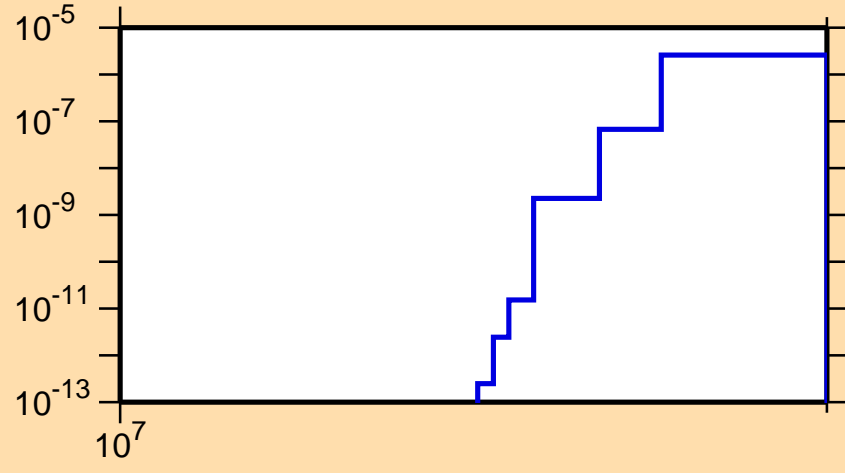
\sigma vs. E for ^{181}\text{Lu}(n,nd)
