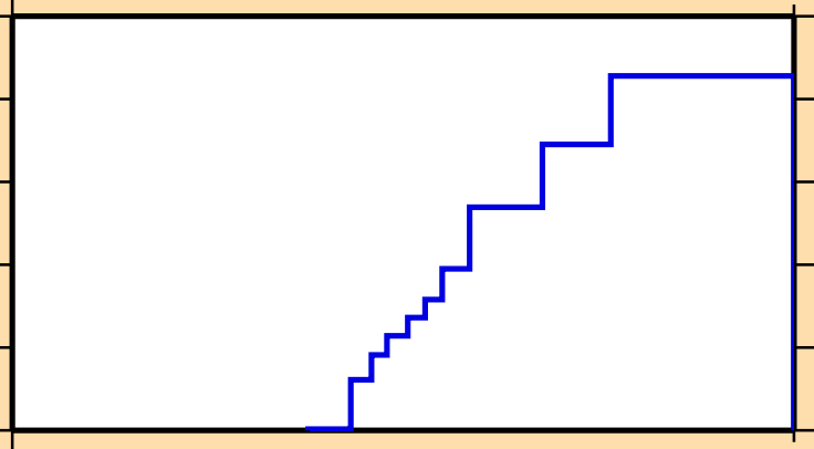
\sigma vs. E for ^{181}\text{Lu}(n,2n\alpha)
