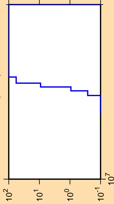
\Delta\sigma/\sigma vs. E for ^{181}\text{Lu}(n,nd)
