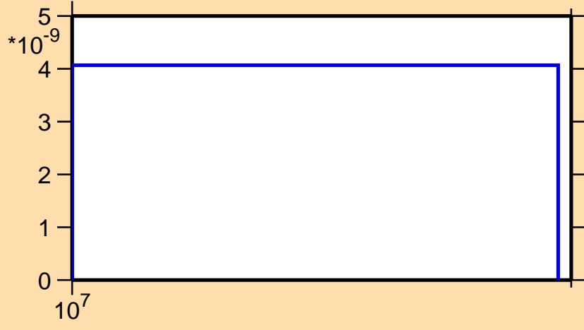
\sigma vs. E for ^{181}\text{Lu}(n,2n\alpha)
