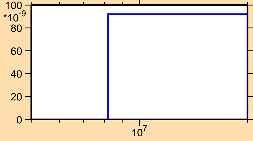
\sigma vs. E for ^{181}\text{Lu}(n,nt)
