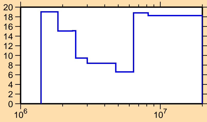
\Delta\sigma/\sigma vs. E for ^{181}\text{Lu}(n,n\text{cont.})
