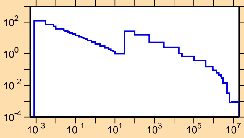
\sigma vs. E for ^{181}\text{Lu}(n,\gamma)
