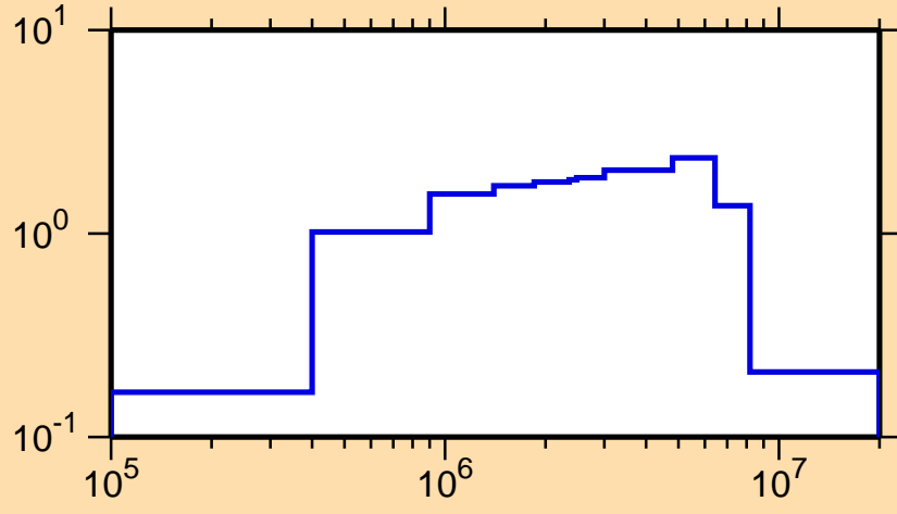
\sigma vs. E for ^{181}\text{Lu}(n,n\text{cont.})
