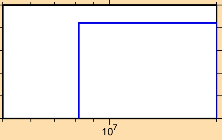
\sigma vs. E for ^{181}\text{Lu}(n,d)
