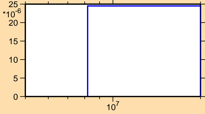
\sigma vs. E for ^{181}\text{Lu}(n,t)
