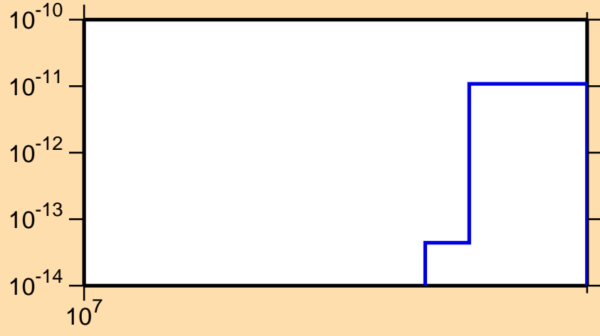
\sigma vs. E for ^{183}\text{Lu}(n,3n\alpha)
