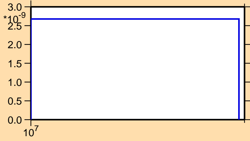
\sigma vs. E for ^{183}\text{Lu}(n,2n\alpha)
