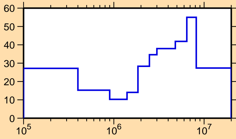
\Delta\sigma/\sigma vs. E for ^{183}\text{Lu}(n, el.)
