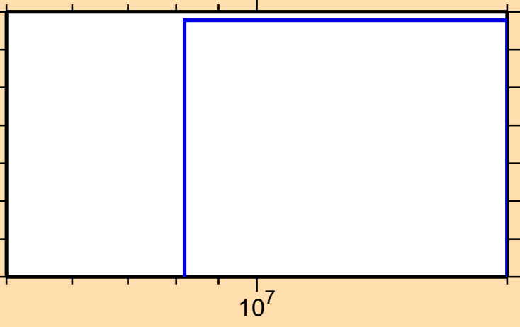
\sigma vs. E for ^{183}\text{Lu}(n,t)
