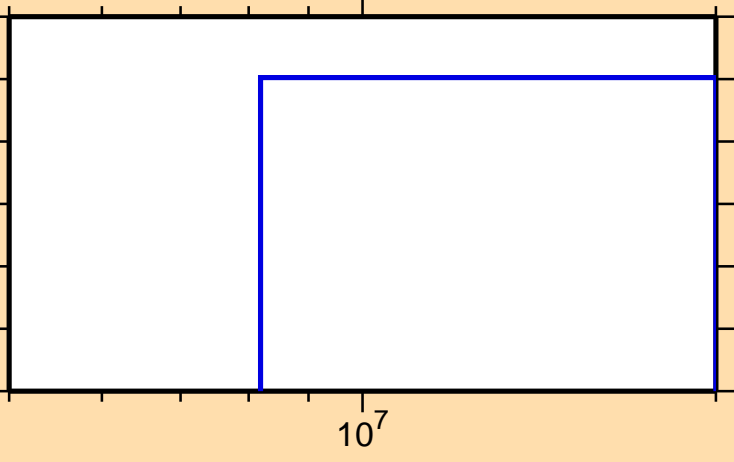
\sigma vs. E for ^{183}\text{Lu}(n,np)
