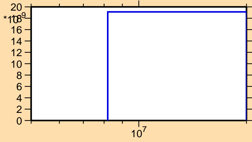
\sigma vs. E for ^{183}\text{Lu}(n,nd)
