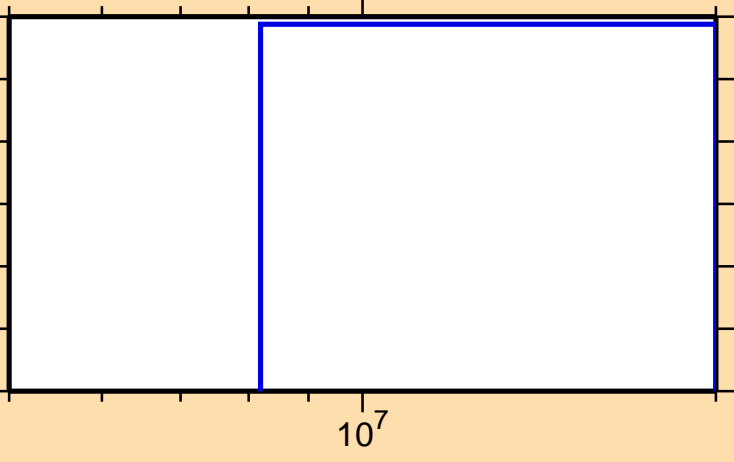
\sigma vs. E for ^{183}\text{Lu}(n,d)
