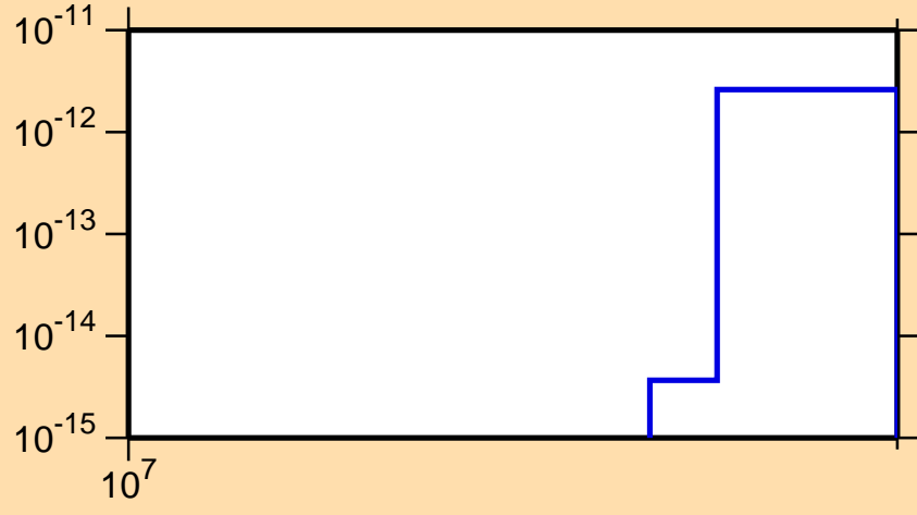
\sigma vs. E for ^{184}\text{Lu}(n,3n\alpha)
