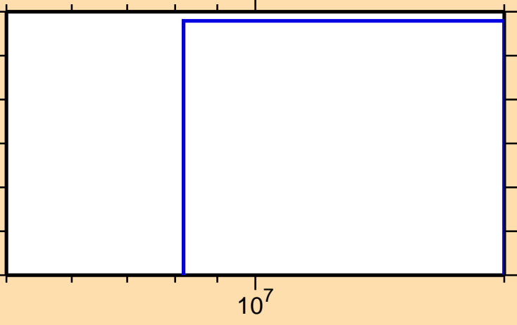
\sigma vs. E for ^{184}\text{Lu}(n,2np)
