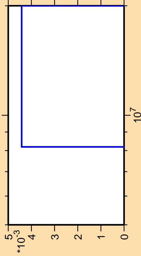
\Delta\sigma/\sigma vs. E for ^{184}\text{Lu} (mt 11)
