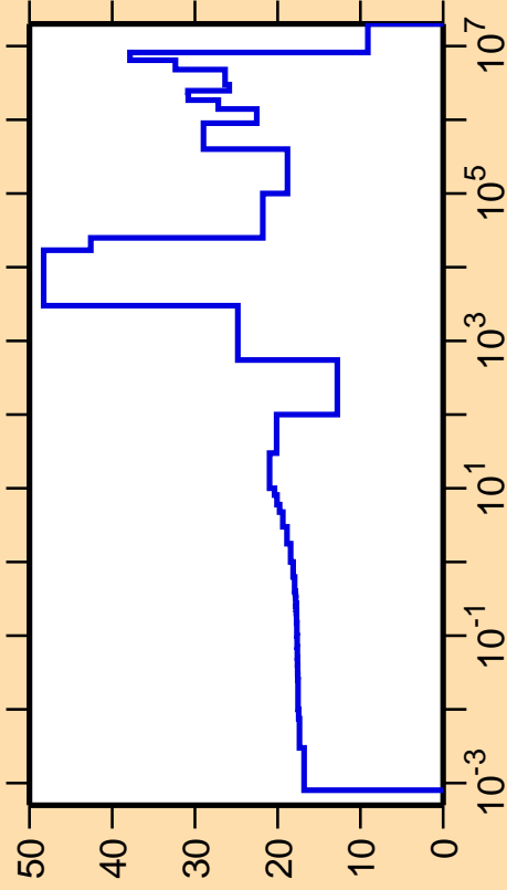
\Delta\sigma/\sigma vs. E for ^{184}\text{Lu}(n,\text{el.})
