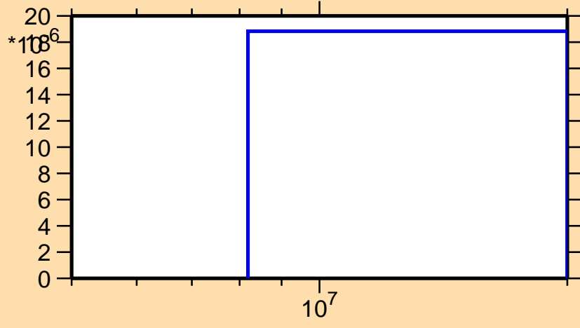
\sigma vs. E for ^{184}\text{Lu}(n,t)
