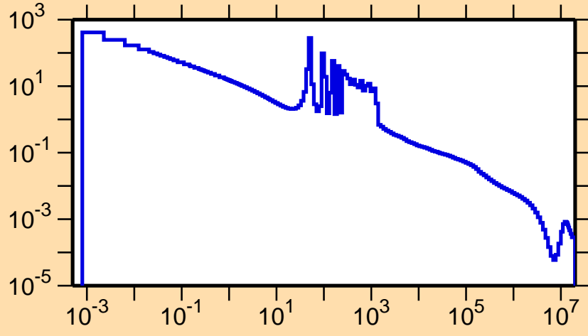
\sigma vs. E for ^{185}\text{Lu}(n,\gamma)
