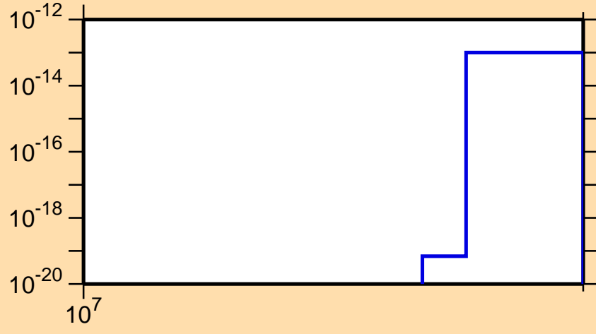
\sigma vs. E for ^{185}\text{Lu} (mt 11)
