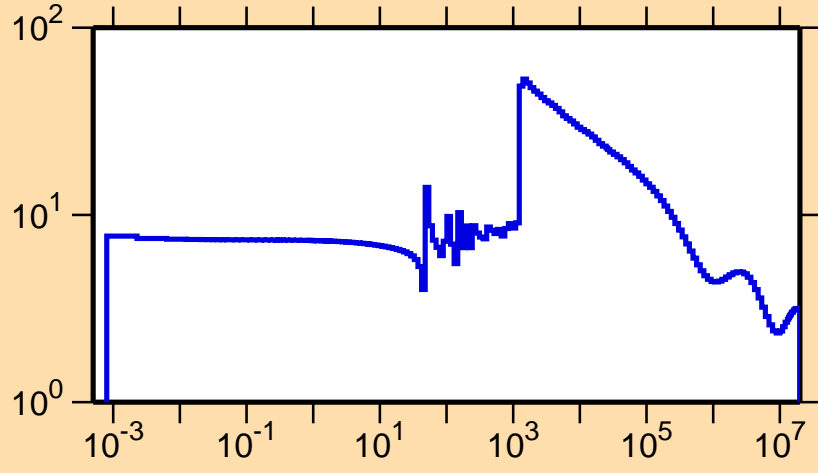
\sigma vs. E for ^{185}\text{Lu}(n,\text{el.})
