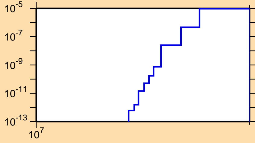
\sigma vs. E for ^{185}\text{Lu}(n,nt)
