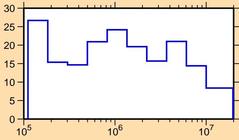
\Delta\sigma/\sigma vs. E for ^{185}\text{Lu}(n, el.)
