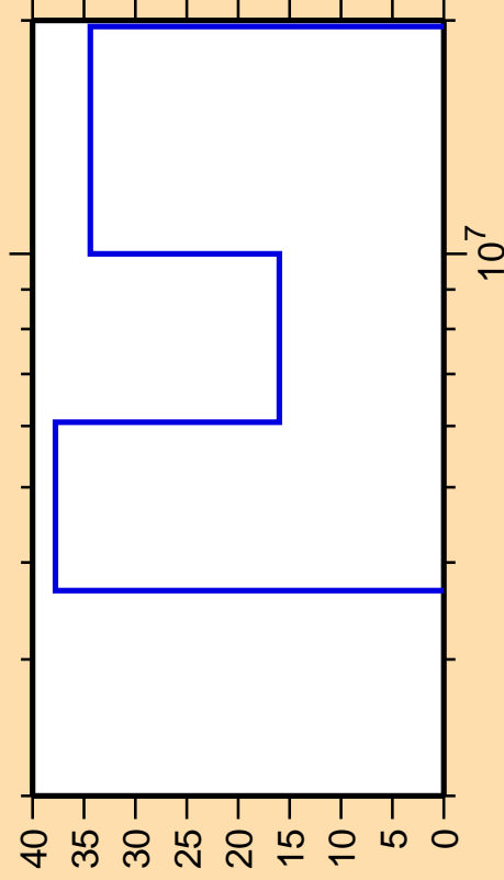
\Delta\sigma/\sigma vs. E for ^{185}\text{Lu}(n,2n)
