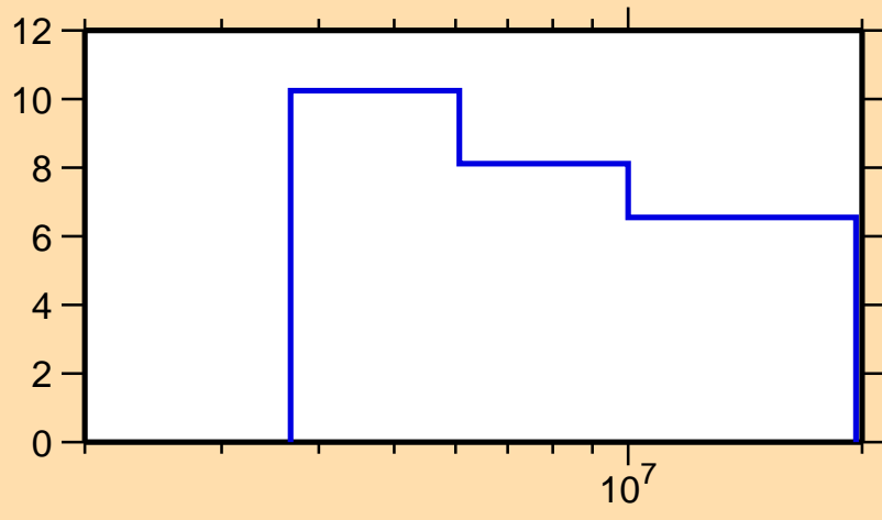
\Delta\sigma/\sigma vs. E for ^{185}\text{Lu}(n,\text{nonel.})
