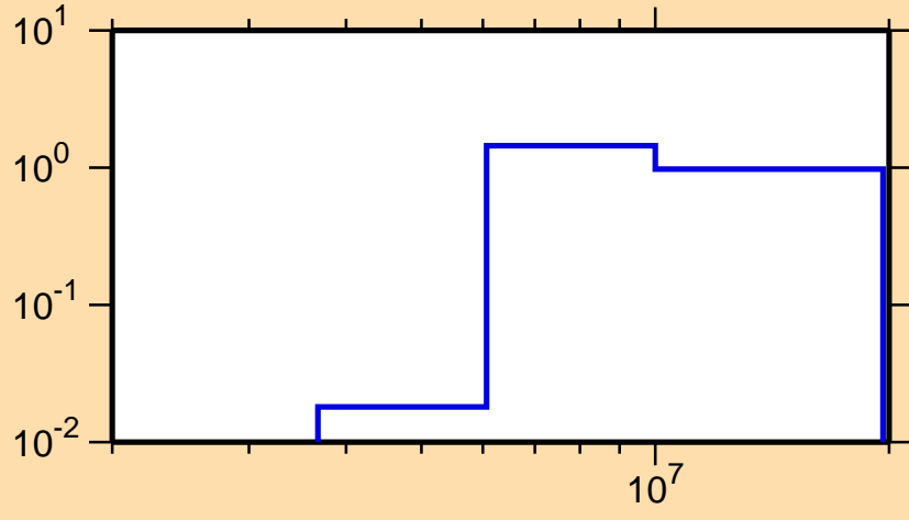
\sigma vs. E for ^{185}\text{Lu}(n,2n)
