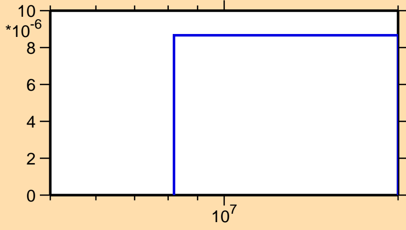
\sigma vs. E for ^{185}\text{Lu}(n,t)
