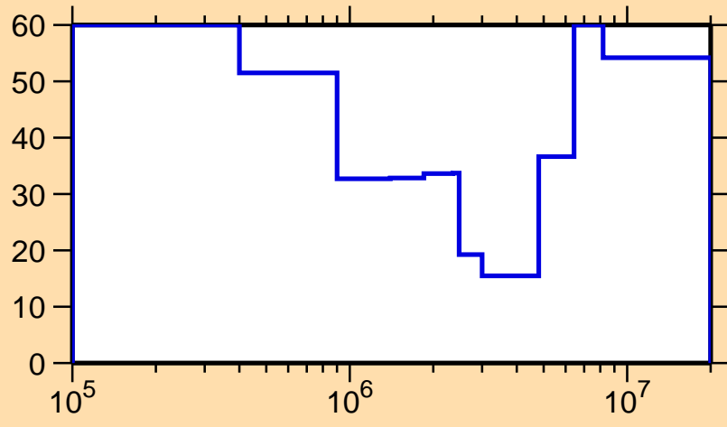
\Delta\sigma/\sigma vs. E for ^{185}\text{Lu}(n,n\text{cont.})
