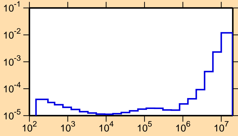
\sigma vs. E for ^{246}\text{Md}(n,p\alpha)
