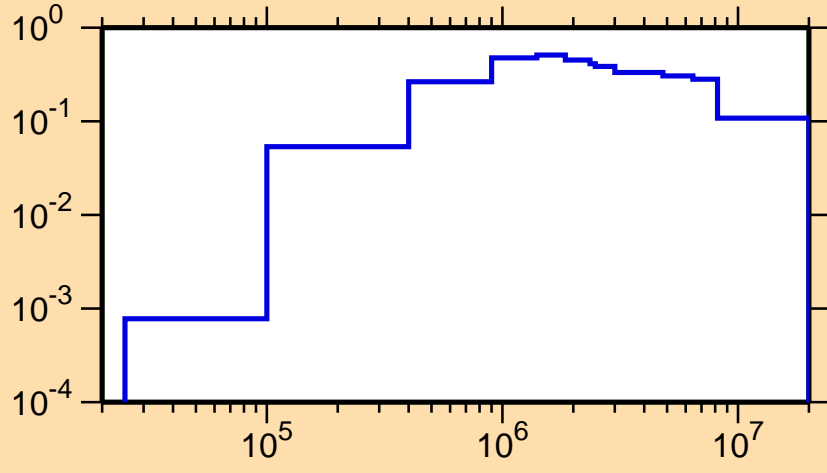
\sigma vs. E for ^{246}\text{Md}(n,n\text{cont.})
