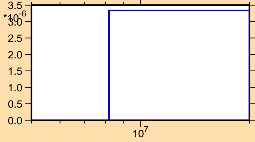
\sigma vs. E for ^{246}\text{Md}(n,3n\alpha)
