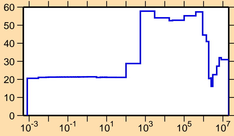
\Delta\sigma/\sigma vs. E for ^{246}\text{Md}(n,el.)
