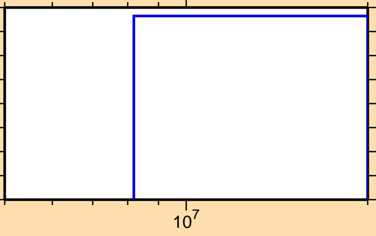
\sigma vs. E for ^{246}\text{Md}(n,nd)
