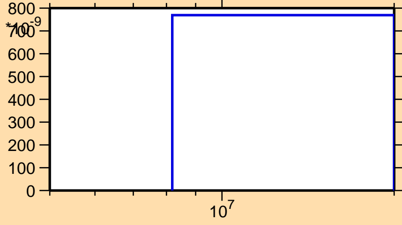
\sigma vs. E for ^{246}\text{Md}(n,2np)
