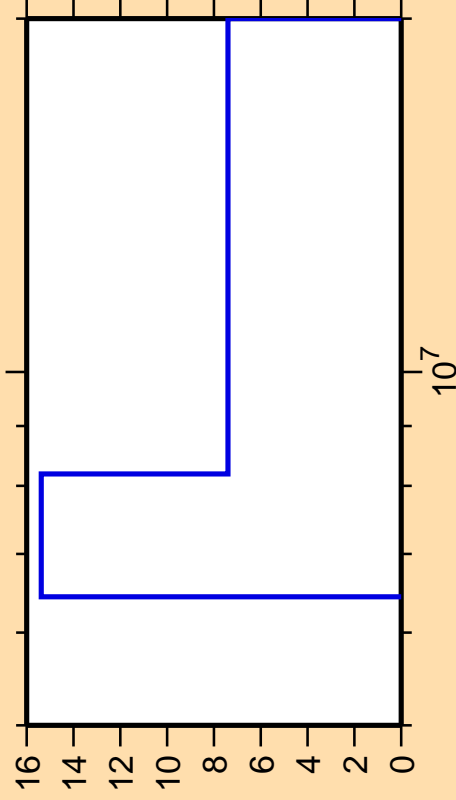
\Delta\sigma/\sigma vs. E for ^{246}\text{Md}(n,f)
