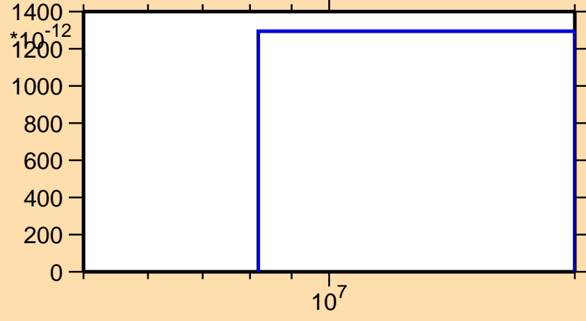
\sigma vs. E for ^{246}\text{Md}(n,nt)
