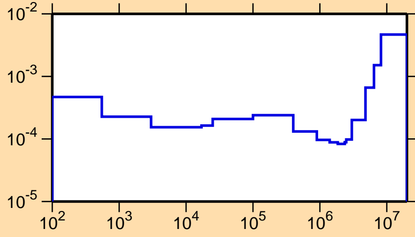
\sigma vs. E for ^{246}\text{Md}(n,p)
