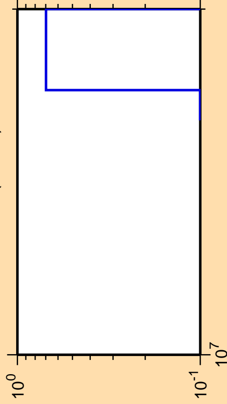
\Delta\sigma/\sigma vs. E for ^{247}\text{Md} (mt 11)
