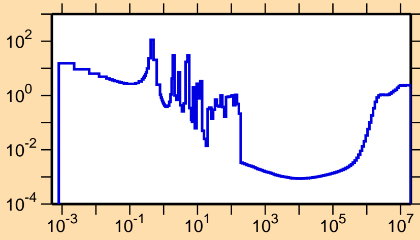
\sigma vs. E for ^{247}\text{Md}(n,f)
