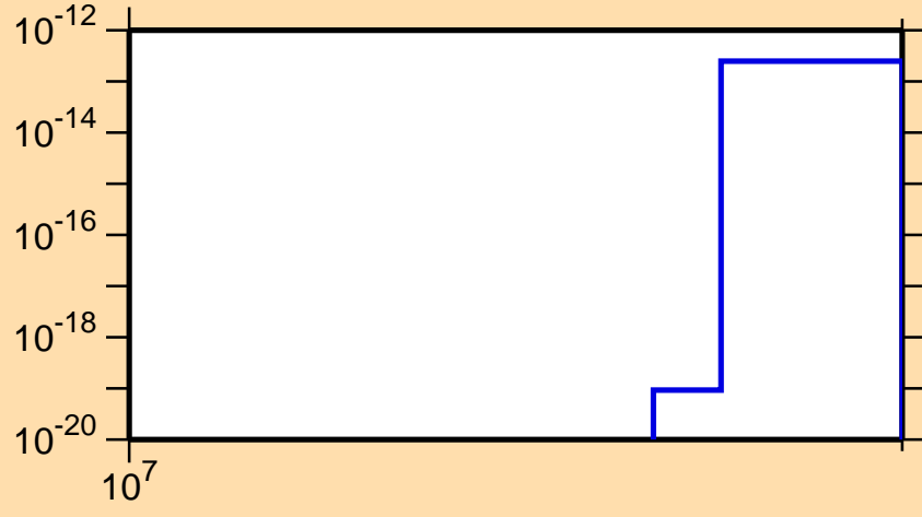
\sigma vs. E for ^{247}\text{Md} (mt 11)
