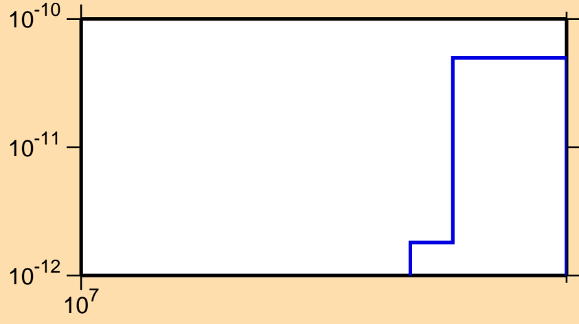
\sigma vs. E for ^{247}\text{Md} (mt 34)
