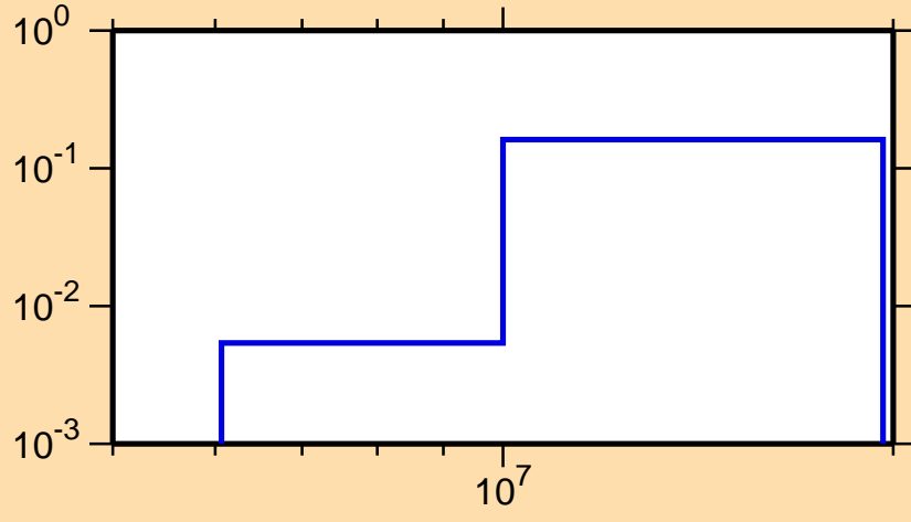
\sigma vs. E for ^{247}\text{Md}(n,2n)
