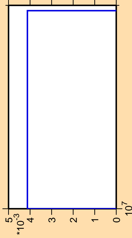
\Delta\sigma/\sigma vs. E for ^{247}\text{Md}(\text{mt } 11)
