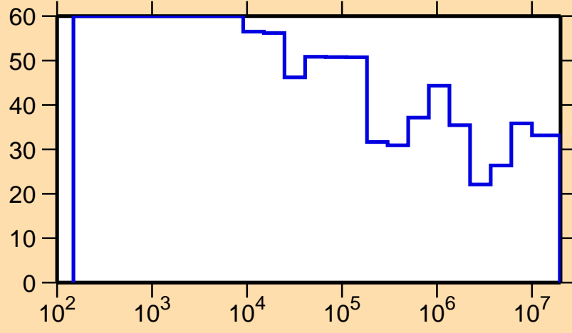
\Delta\sigma/\sigma vs. E for ^{247}\text{Md}(n,\text{el.})
