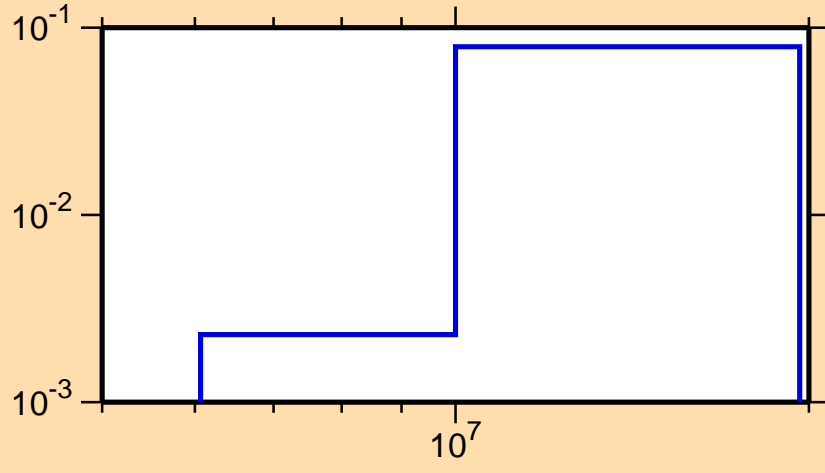
\sigma vs. E for ^{247}\text{Md}(n,2n\alpha)
