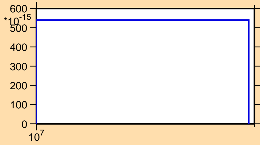
\sigma vs. E for ^{247}\text{Md} (mt 34)
