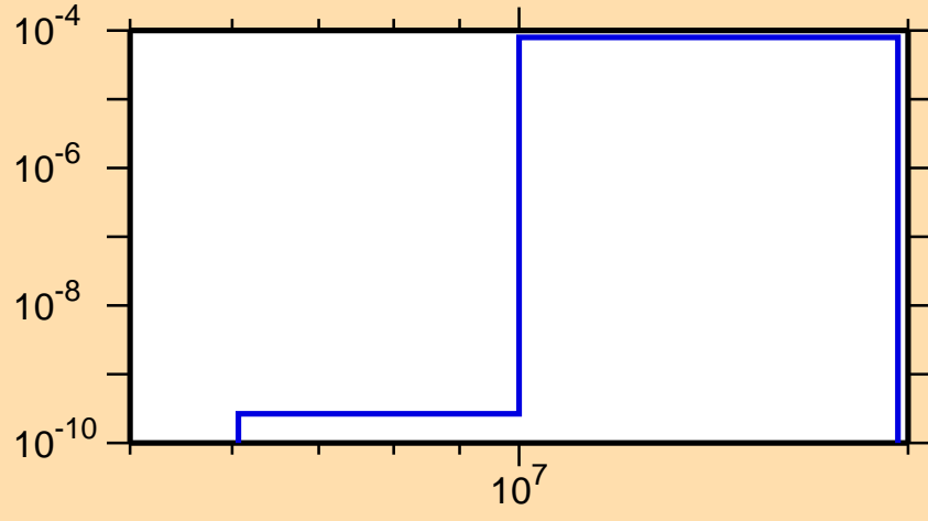
\sigma vs. E for ^{247}\text{Md}(n,t)
