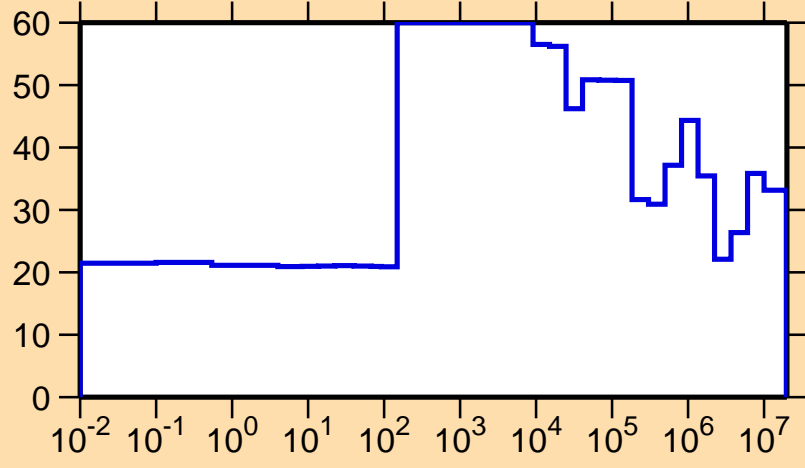
\Delta\sigma/\sigma vs. E for ^{247}\text{Md}(n,el.)
