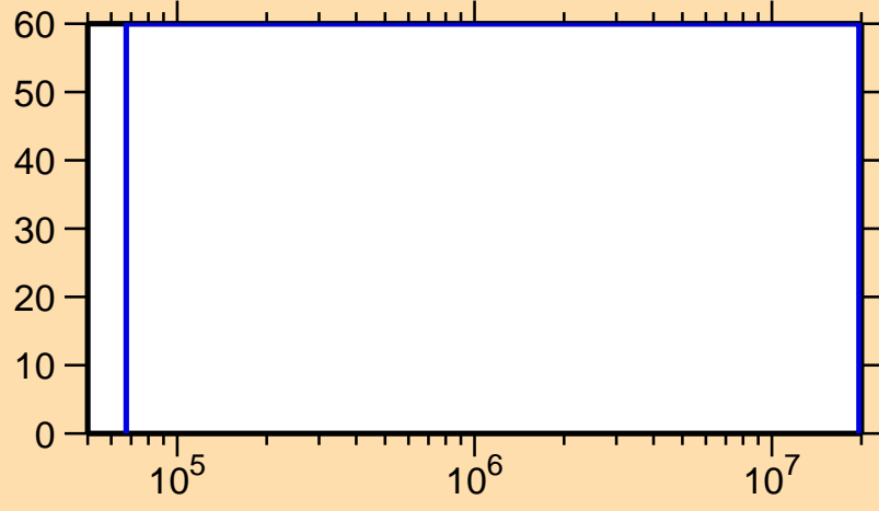
\Delta\sigma/\sigma vs. E for ^{247}\text{Md}(n,n_1)
