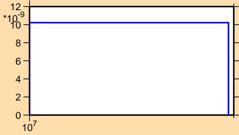
\sigma vs. E for ^{247}\text{Md}(n,nt)
