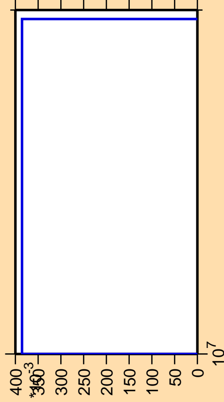
\Delta\sigma/\sigma vs. E for ^{247}\text{Md} (mt 34)
