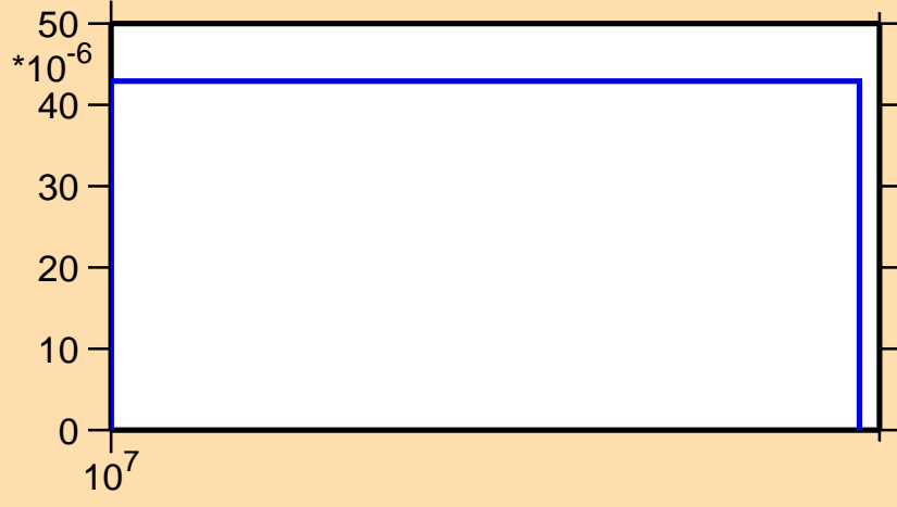
\sigma vs. E for ^{247}\text{Md}(n,3n\alpha)
