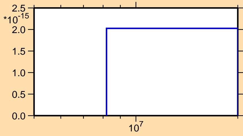
\sigma vs. E for ^{247}\text{Md}(\text{mt } 11)
