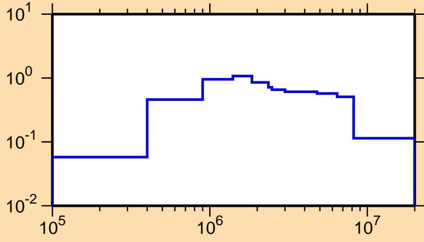
\sigma vs. E for ^{247}\text{Md}(n,n\text{cont.})
