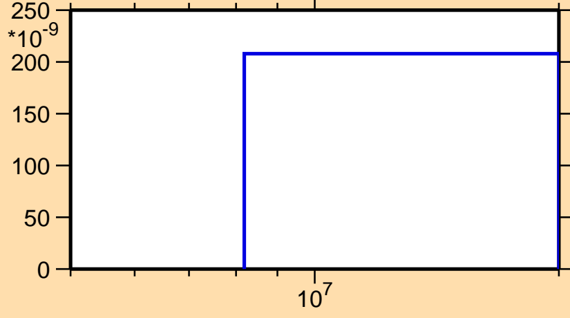
\sigma vs. E for ^{247}\text{Md}(n,2np)
