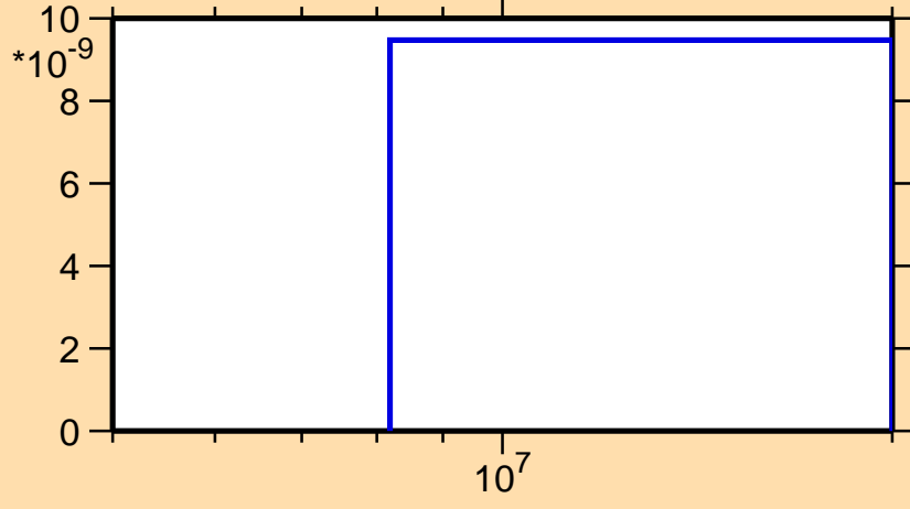
\sigma vs. E for ^{247}\text{Md}(n,\text{He3})
