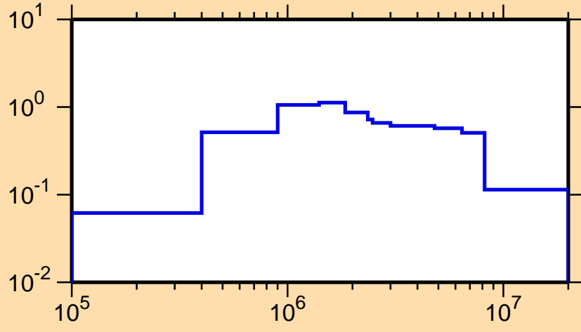
\sigma vs. E for ^{247}\text{Md}(n,\text{inel.})
