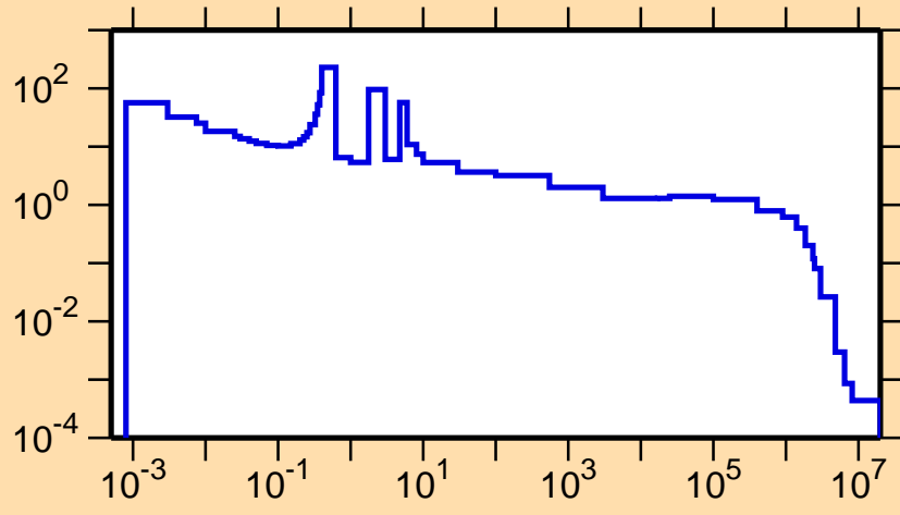
\sigma vs. E for ^{247}\text{Md}(n,\gamma)
