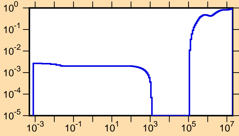
\mu vs. E for ^{248}\text{Md}(\text{mt251})
