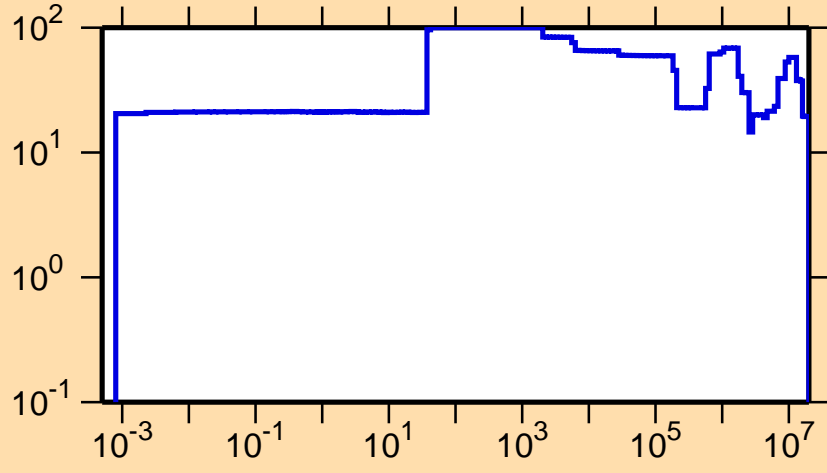
\Delta\sigma/\sigma vs. E for ^{248}\text{Md}(n,el.)
