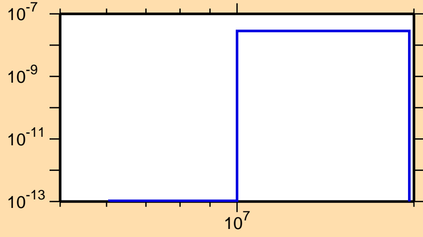
\sigma vs. E for ^{248}\text{Md}(n,\text{He3})
