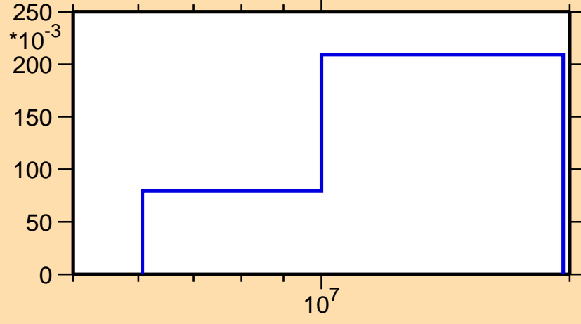
\sigma vs. E for ^{248}\text{Md}(n,2n)
