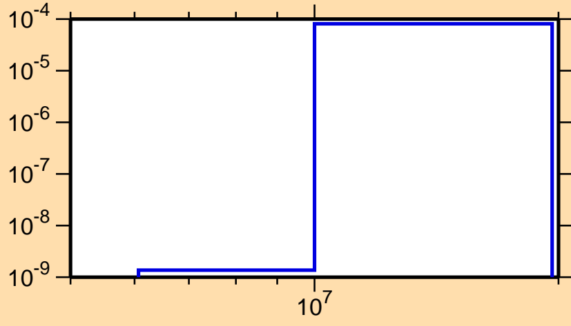
\sigma vs. E for ^{248}\text{Md}(n,t)
