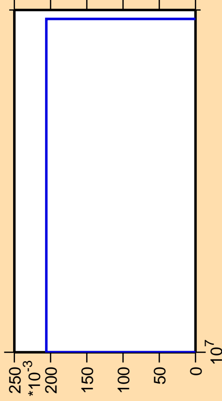
\Delta\sigma/\sigma vs. E for ^{248}\text{Md}(n,\text{pd})
