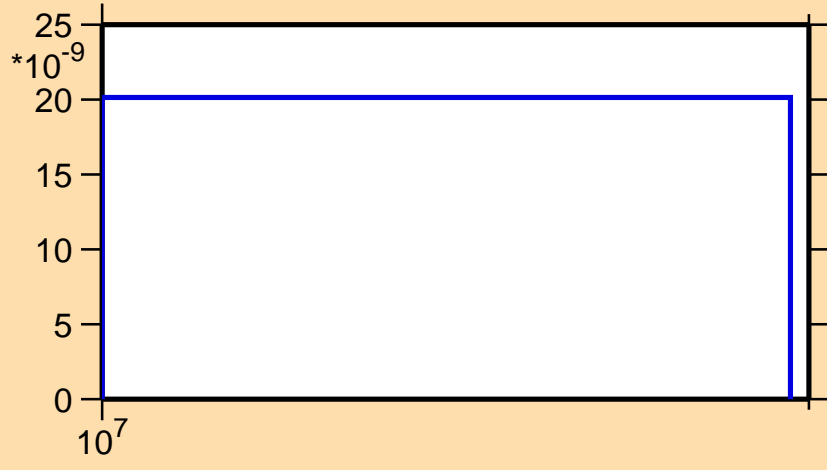
\sigma vs. E for ^{248}\text{Md}(n,nt)
