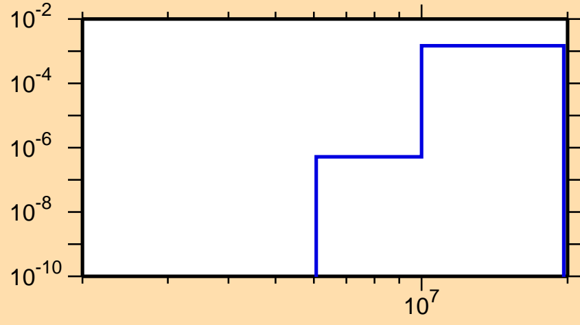
\sigma vs. E for ^{248}\text{Md}(n,d)
