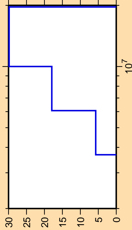
\Delta\sigma/\sigma vs. E for ^{248}\text{Md}(n,d)
