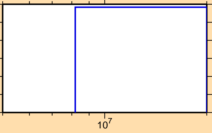
\sigma vs. E for ^{248}\text{Md}(n,3n)
