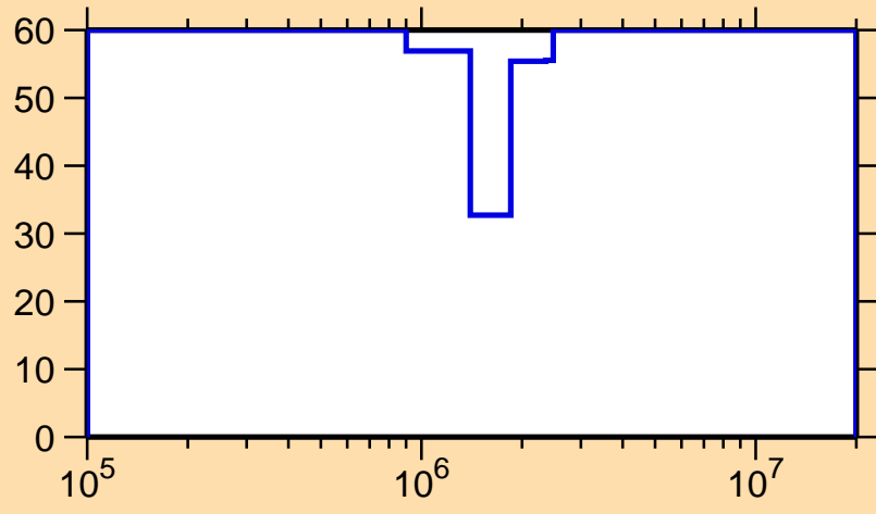
\Delta\sigma/\sigma vs. E for ^{248}\text{Md}(n,n_1)
