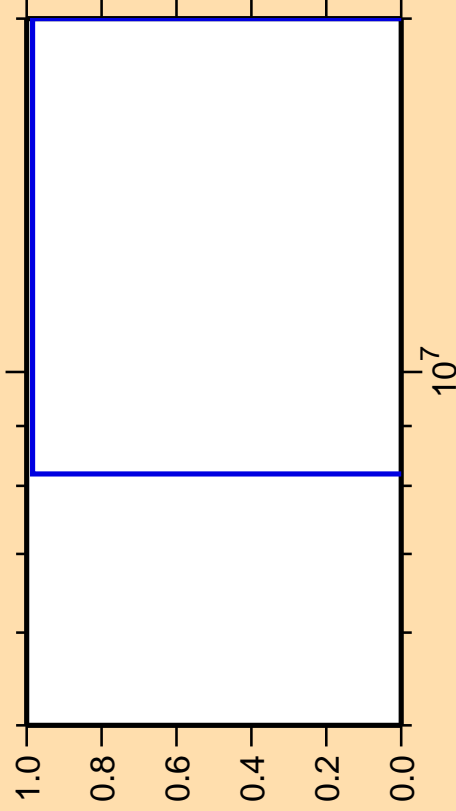
\Delta\sigma/\sigma vs. E for ^{248}\text{Md}(\text{mt } 34)
