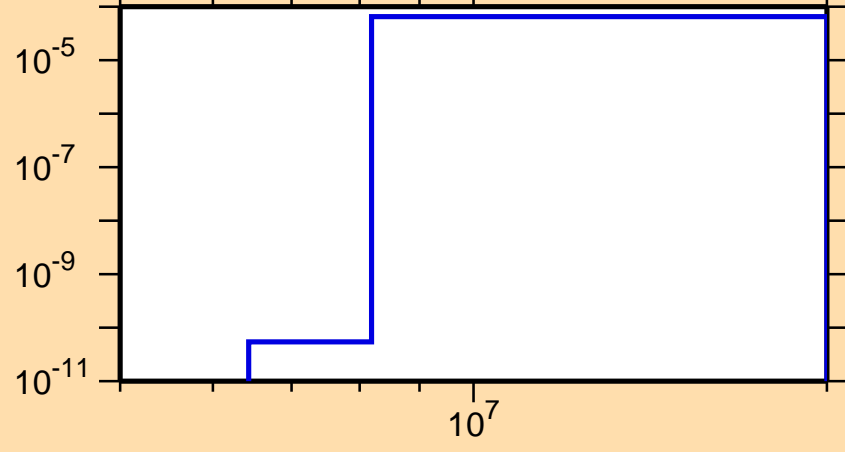
\sigma vs. E for ^{248}\text{Md}(n,t)
