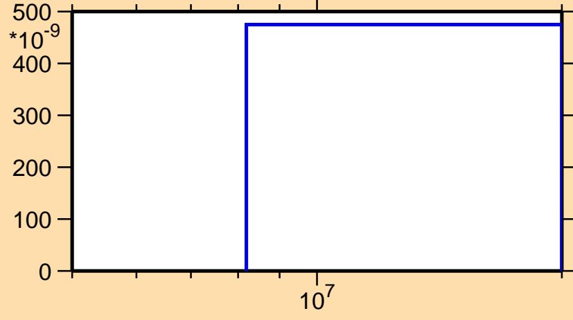
\sigma vs. E for ^{248}\text{Md}(n,\text{nd})
