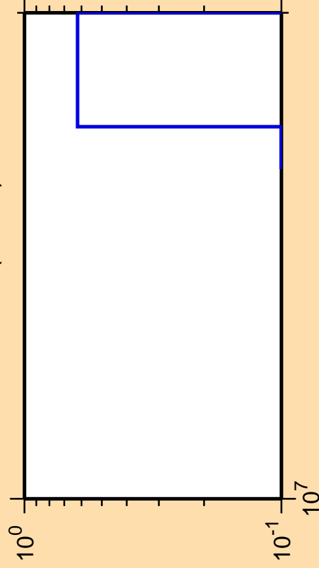
\Delta\sigma/\sigma vs. E for ^{249}\text{Md} (mt 11)
