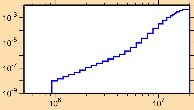
\sigma vs. E for ^{249}\text{Md}(n,p\alpha)
