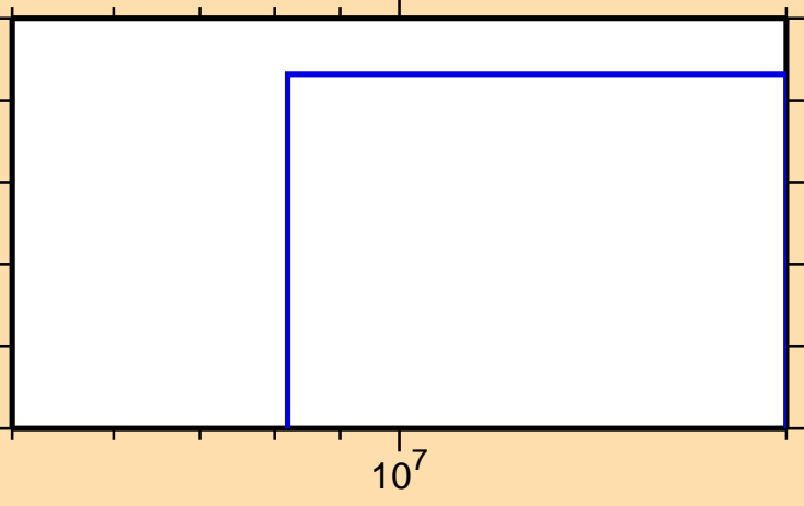
\sigma vs. E for ^{249}\text{Md}(n,nd)
