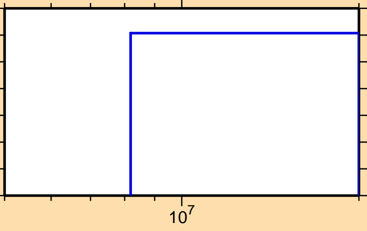
\sigma vs. E for ^{249}\text{Md}(n,nt)
