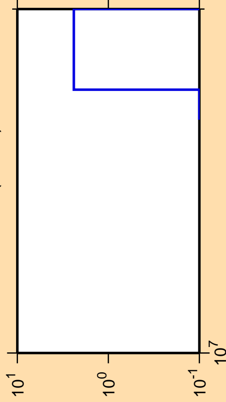
\Delta\sigma/\sigma vs. E for ^{249}\text{Md} (mt 42)
