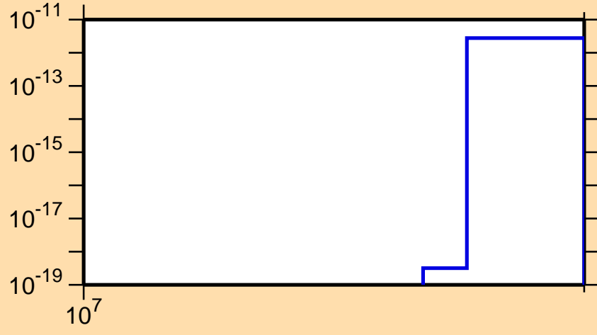
\sigma vs. E for ^{249}\text{Md} (mt 42)
