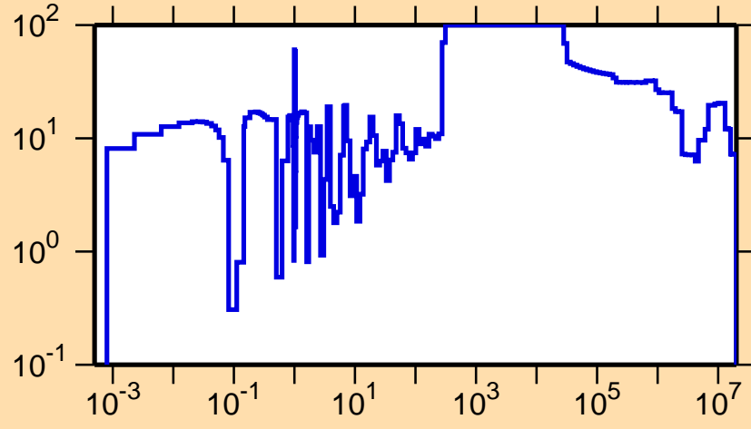
\Delta\sigma/\sigma vs. E for ^{249}\text{Md}(n,tot.)
