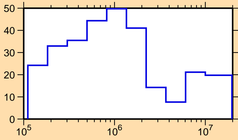
\Delta\sigma/\sigma vs. E for ^{249}\text{Md}(n, el.)
