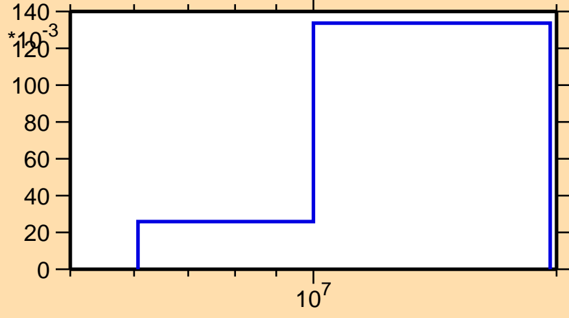
\sigma vs. E for ^{249}\text{Md}(n,2n)
