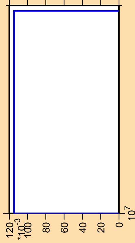
\Delta\sigma/\sigma vs. E for ^{249}\text{Md} (mt 34)
