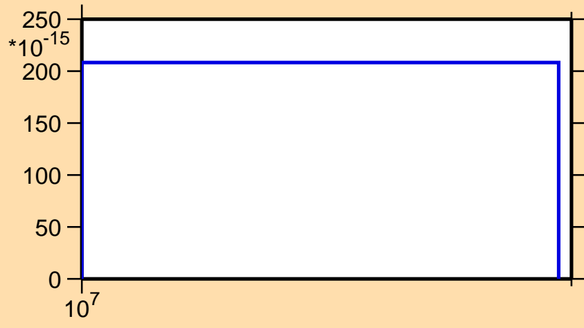
\sigma vs. E for ^{249}\text{Md} (mt 34)
