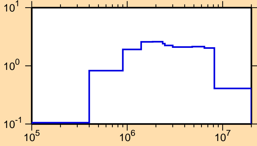
\sigma vs. E for ^{249}\text{Md}(n,n\text{cont.})
