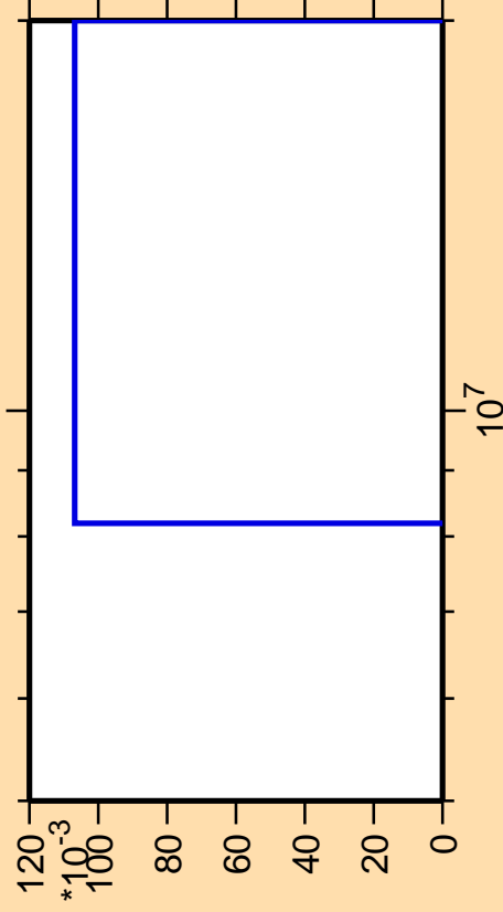
\Delta\sigma/\sigma vs. E for ^{249}\text{Md}(\text{mt } 34)
