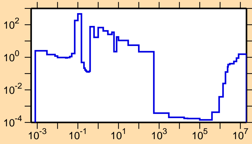
\sigma vs. E for ^{249}\text{Md}(n,f)
