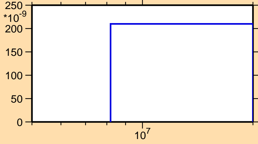
\sigma vs. E for ^{249}\text{Md}(n,nd)
