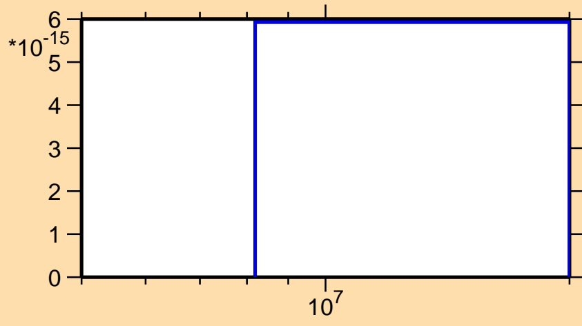
\sigma vs. E for ^{249}\text{Md} (mt 11)
