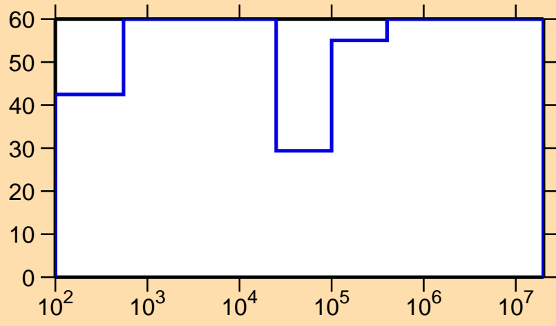
\Delta\sigma/\sigma vs. E for ^{249}\text{Md}(n,p)
