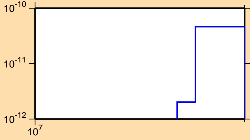
\sigma vs. E for ^{250}\text{Md} (mt 34)
