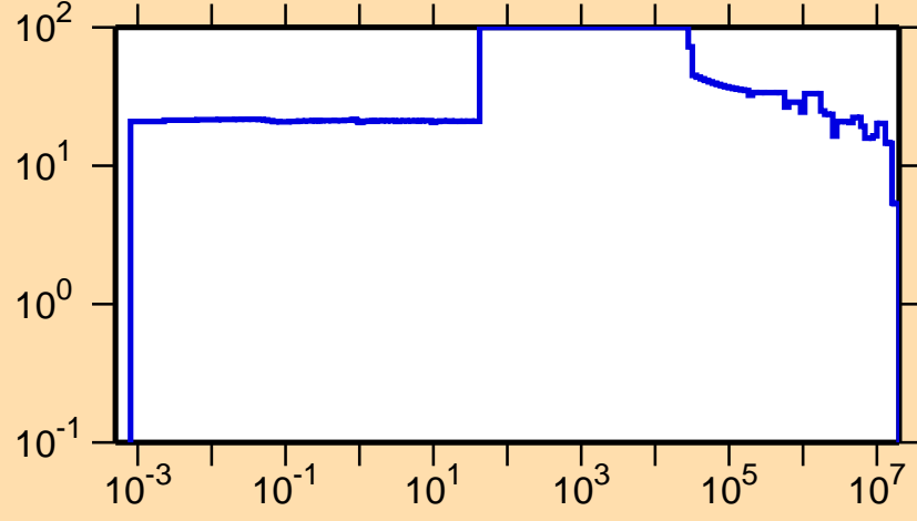
\Delta\sigma/\sigma vs. E for ^{250}\text{Md}(n,el.)
