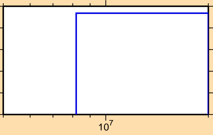
\sigma vs. E for ^{250}\text{Md}(\text{mt } 11)
