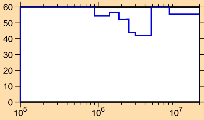
\Delta\sigma/\sigma vs. E for ^{250}\text{Md}(n,ncont.)
