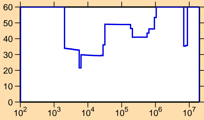
\Delta\sigma/\sigma vs. E for ^{251}\text{Md}(n,\gamma)
