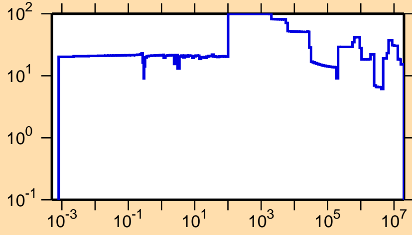
\Delta\sigma/\sigma vs. E for ^{251}\text{Md}(n,el.)
