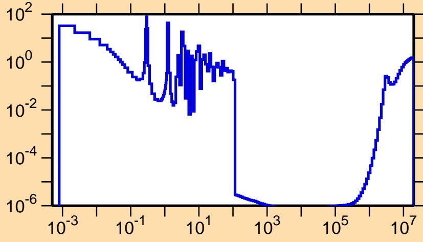
\sigma vs. E for ^{251}\text{Md}(n,f)
