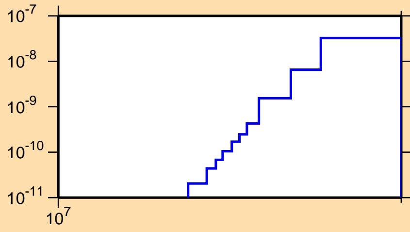
\sigma vs. E for ^{251}\text{Md}(n,\text{He3})
