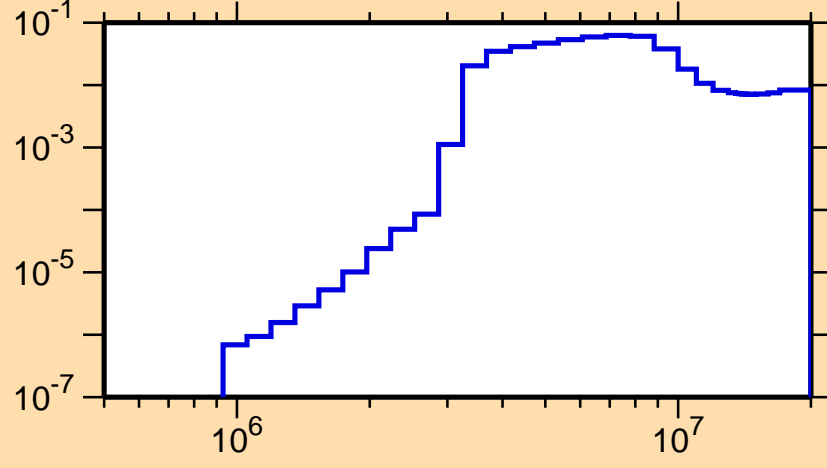
\sigma vs. E for ^{251}\text{Md}(n,n\alpha)
