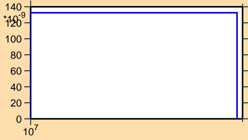
\sigma vs. E for ^{251}\text{Md}(n,\text{nd})
