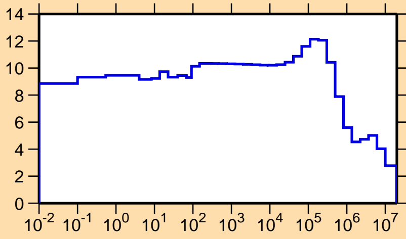
\sigma vs. E for ^{251}\text{Md}(n,\text{el.})
