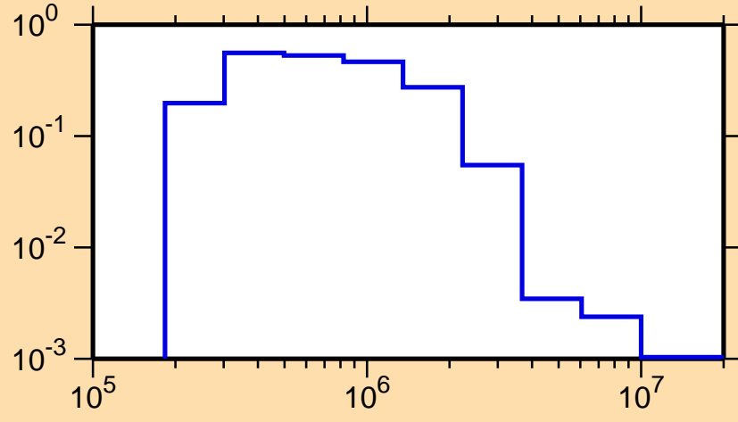
\sigma vs. E for ^{251}\text{Md}(n,n_4)
