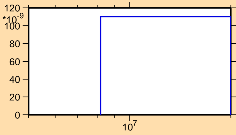
\sigma vs. E for ^{251}\text{Md}(n,nd)
