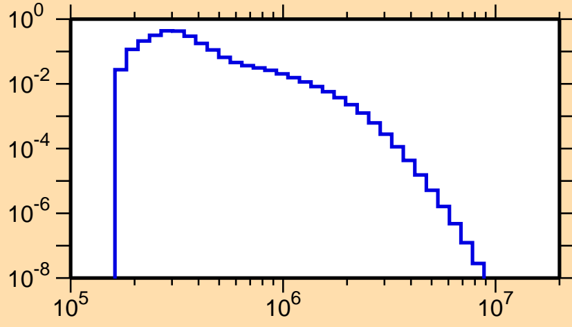
\sigma vs. E for ^{252}\text{Md}(n,n_2)
