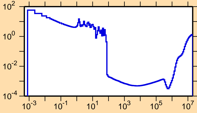
\sigma vs. E for ^{252}\text{Md}(n,f)
