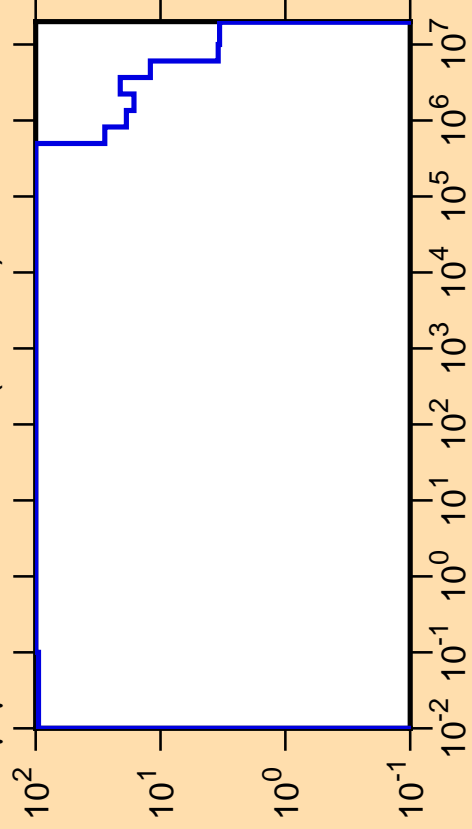
\Delta\mu/\mu vs. E for ^{252}\text{Md}(\text{mt251})
