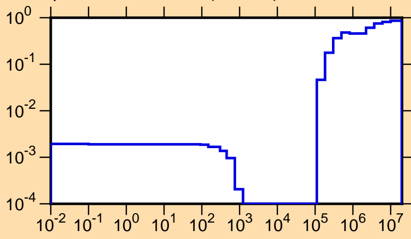
\mu vs. E for ^{252}\text{Md}(\text{mt251})
