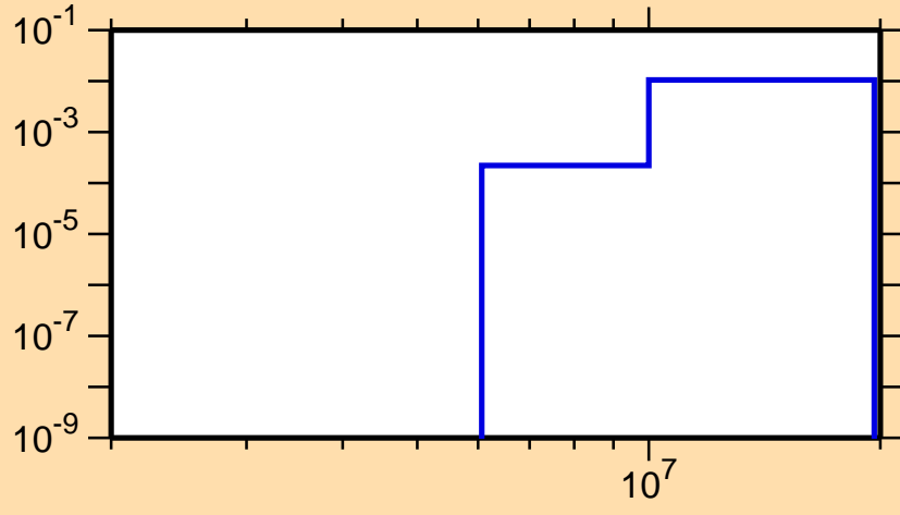
\sigma vs. E for ^{252}\text{Md}(n,2n\alpha)
