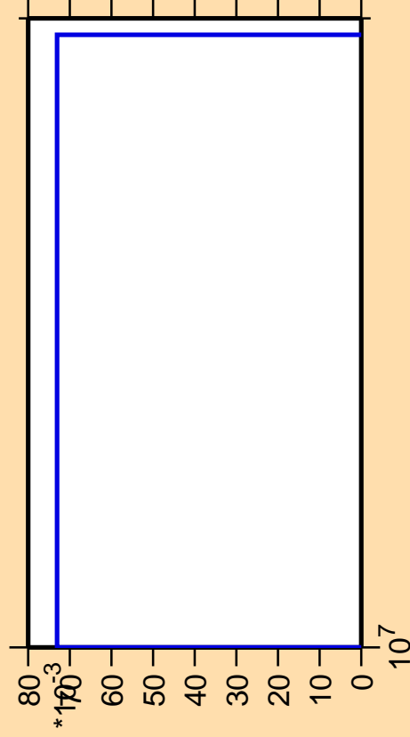
\Delta\sigma/\sigma vs. E for ^{252}\text{Md} (mt 34)
