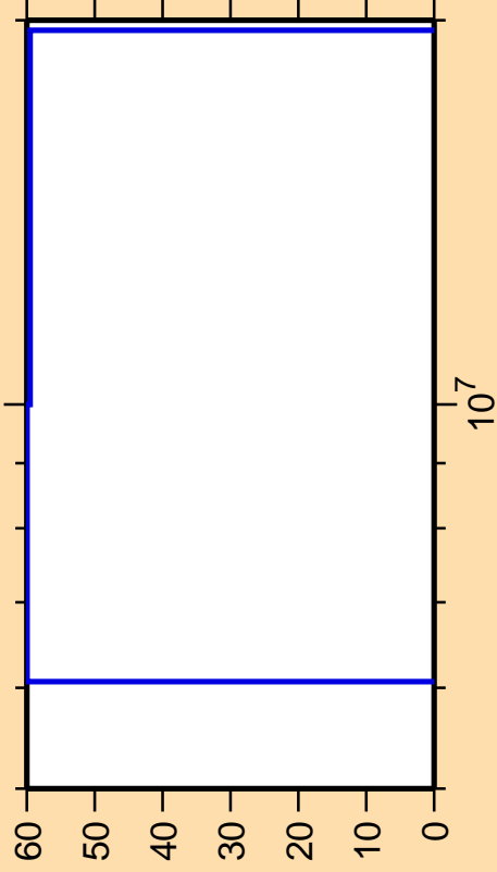
\Delta\sigma/\sigma vs. E for ^{252}\text{Md}(n,t)
