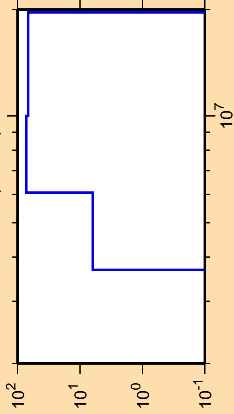
\Delta\sigma/\sigma vs. E for ^{252}\text{Md}(n,2n\alpha)
