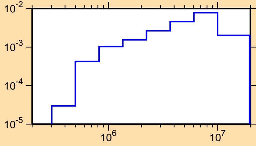
\sigma vs. E for ^{252}\text{Md}(n,n\alpha)
