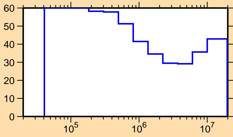
\Delta\sigma/\sigma vs. E for ^{252}\text{Md}(n,\text{inel.})
