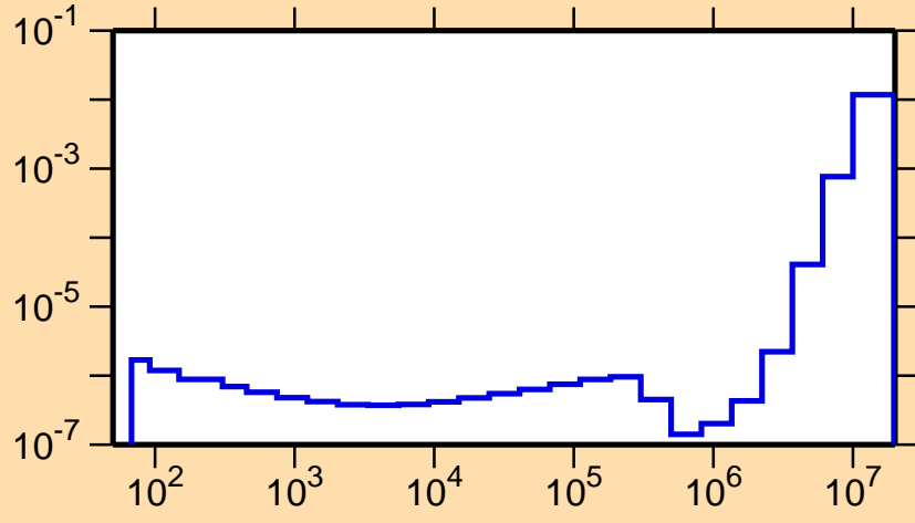
\sigma vs. E for ^{252}\text{Md}(n,p)
