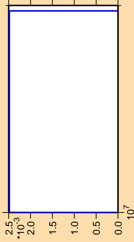
\Delta\sigma/\sigma vs. E for ^{252}\text{Md} (mt 11)
