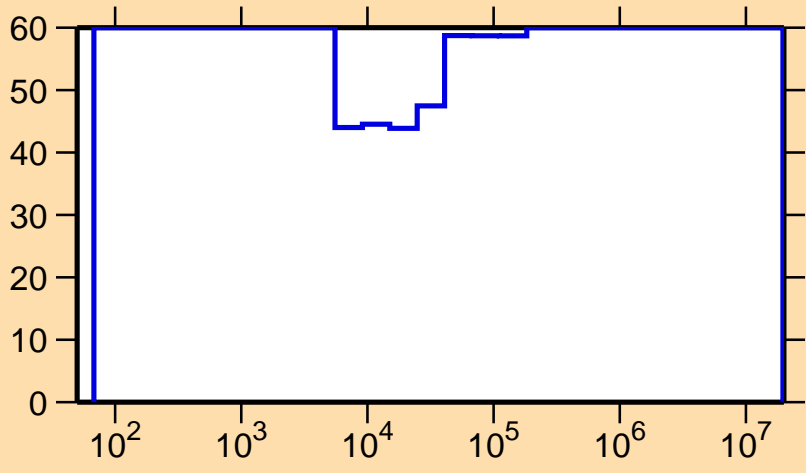
\Delta\sigma/\sigma vs. E for ^{252}\text{Md}(n,\gamma)
