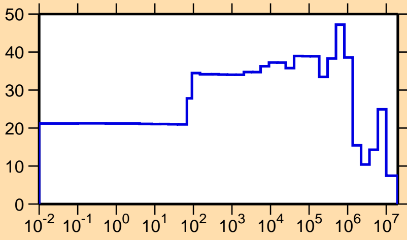
\Delta\sigma/\sigma vs. E for ^{252}\text{Md}(n,\text{el.})
