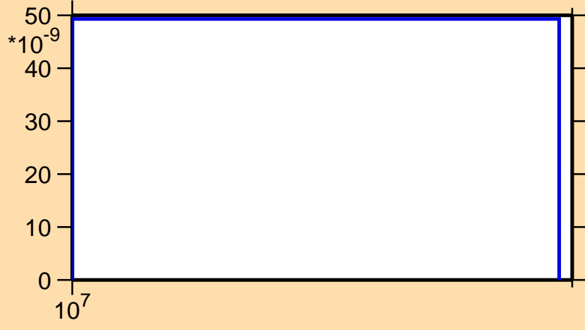
\sigma vs. E for ^{252}\text{Md}(n,nt)
