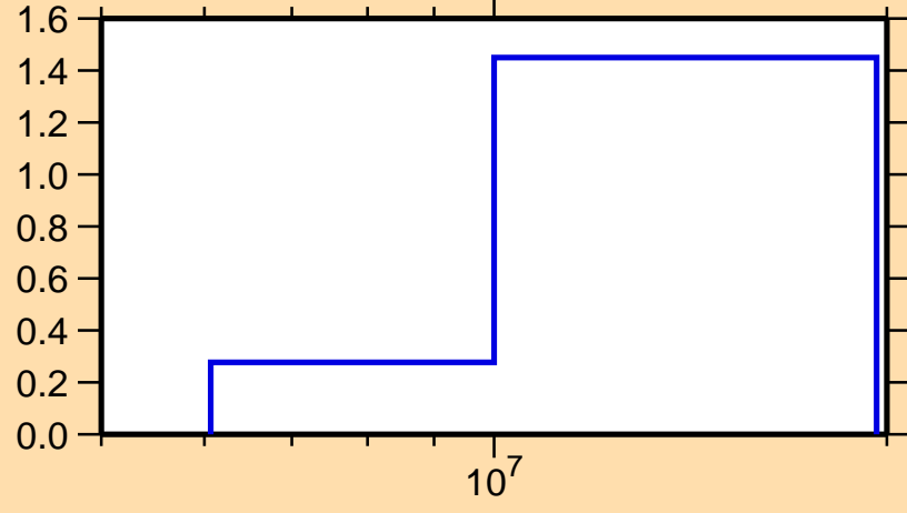
\sigma vs. E for ^{252}\text{Md}(n,2n)
