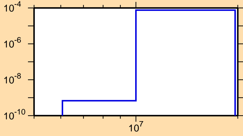
\sigma vs. E for ^{252}\text{Md}(n,t)
