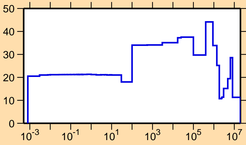
\Delta\sigma/\sigma vs. E for ^{252}\text{Md}(n,el.)
