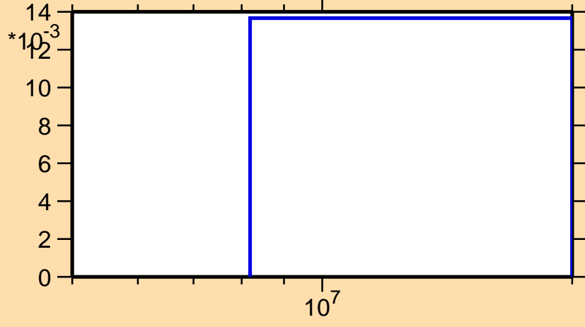
\sigma vs. E for ^{252}\text{Md}(n,3n)
