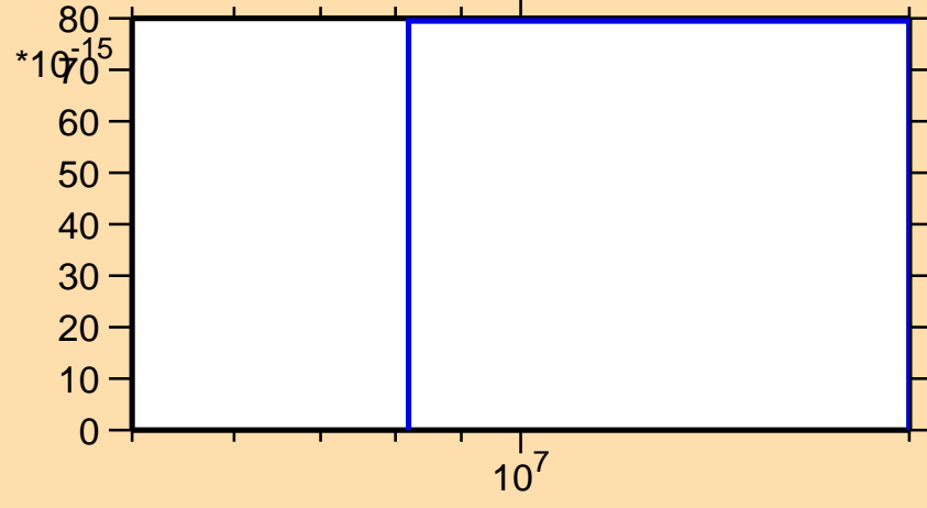
\sigma vs. E for ^{252}\text{Md}(\text{mt } 34)
