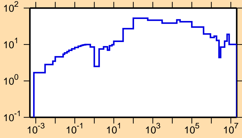
\Delta\sigma/\sigma vs. E for ^{252}\text{Md}(n,tot.)
