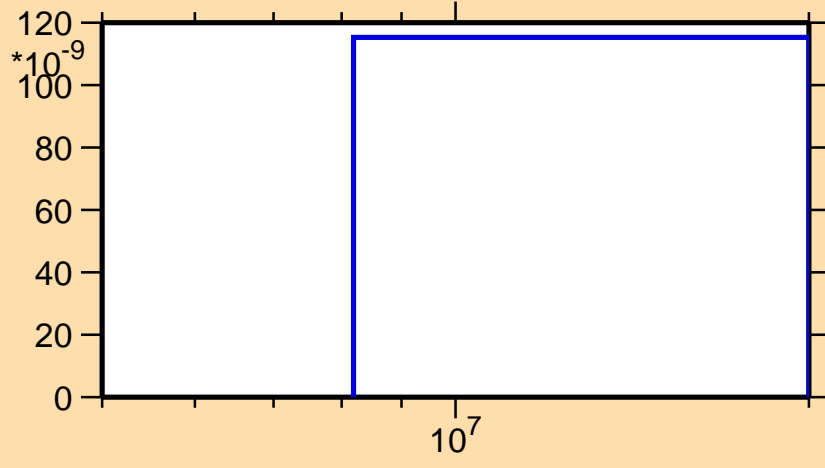
\sigma vs. E for ^{252}\text{Md}(n,nd)
