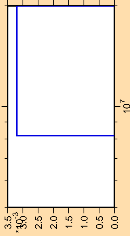
\Delta\sigma/\sigma vs. E for ^{252}\text{Md}(\text{mt } 11)
