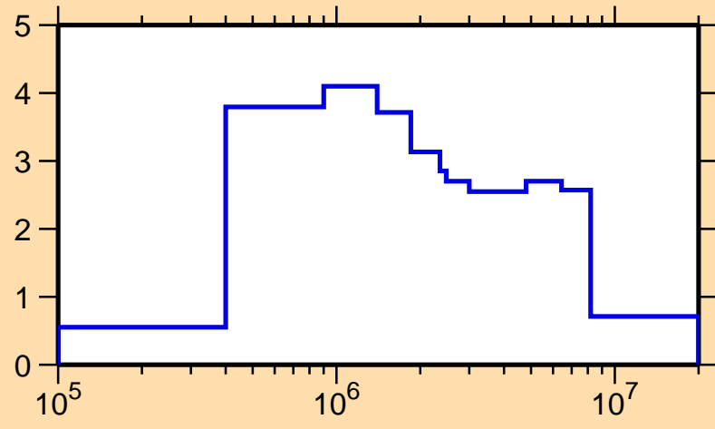
\sigma vs. E for ^{252}\text{Md}(n,\text{inel.})
