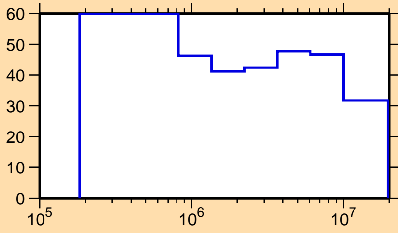
\Delta\sigma/\sigma vs. E for ^{254}\text{Md}(n,n\text{cont.})
