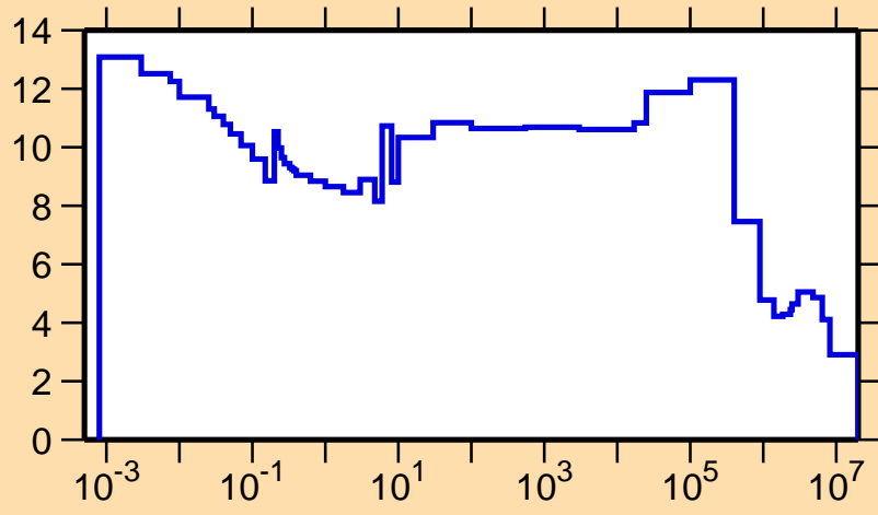
\sigma vs. E for ^{254}\text{Md}(n,\text{el.})
