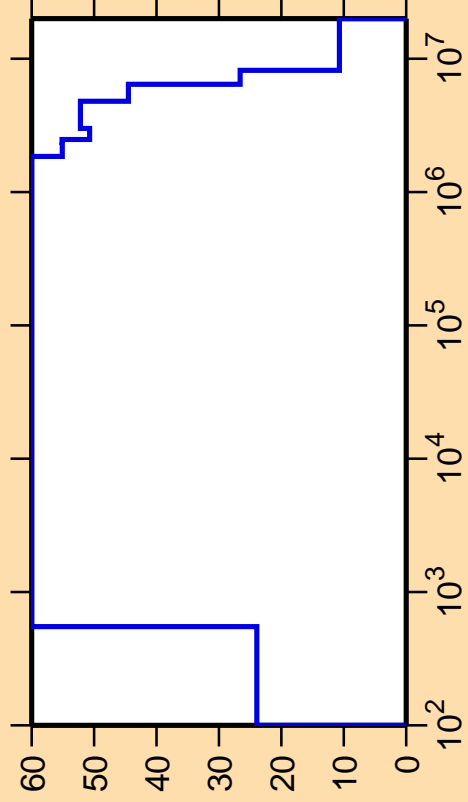
\Delta\sigma/\sigma vs. E for ^{254}\text{Md}(n,\alpha)
