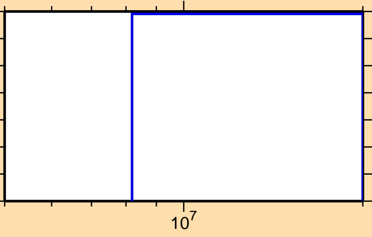
\sigma vs. E for ^{254}\text{Md}(n,3n\alpha)
