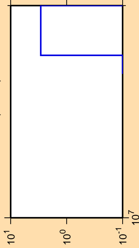
\Delta\sigma/\sigma vs. E for ^{254}\text{Md} (mt 34)
