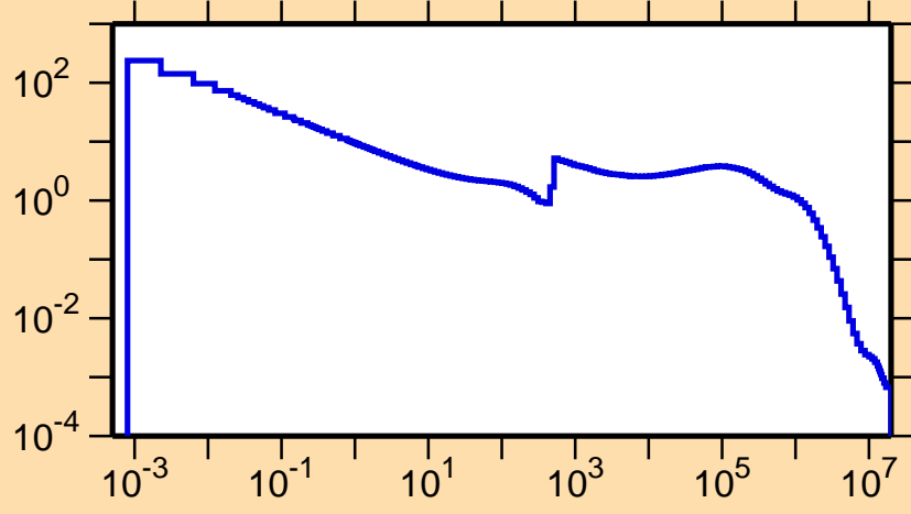
\sigma vs. E for ^{254}\text{Md}(n,\gamma)
