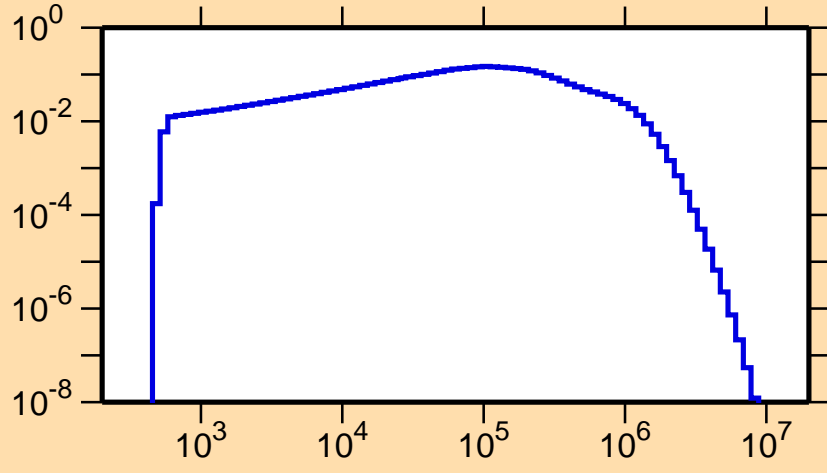
\sigma vs. E for ^{254}\text{Md}(n,n_3)
