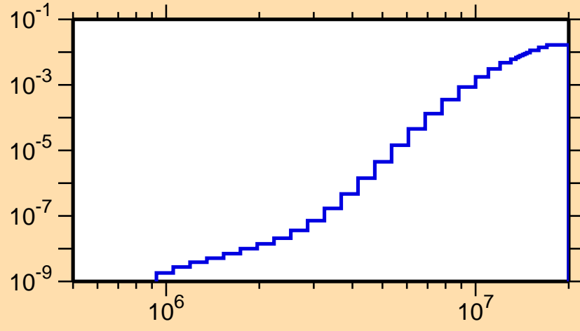
\sigma vs. E for ^{254}\text{Md}(n,p)
