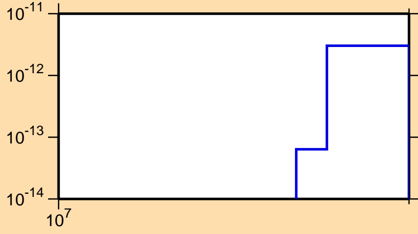
\sigma vs. E for ^{254}\text{Md} (mt 34)
