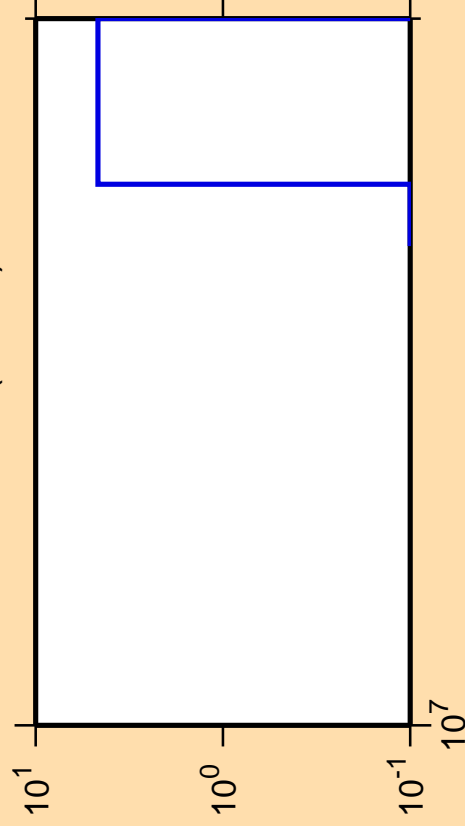
\Delta\sigma/\sigma vs. E for ^{254}\text{Md} (mt 11)
