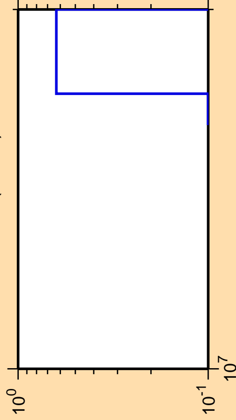
\Delta\sigma/\sigma vs. E for ^{254}\text{Md} (mt 42)
