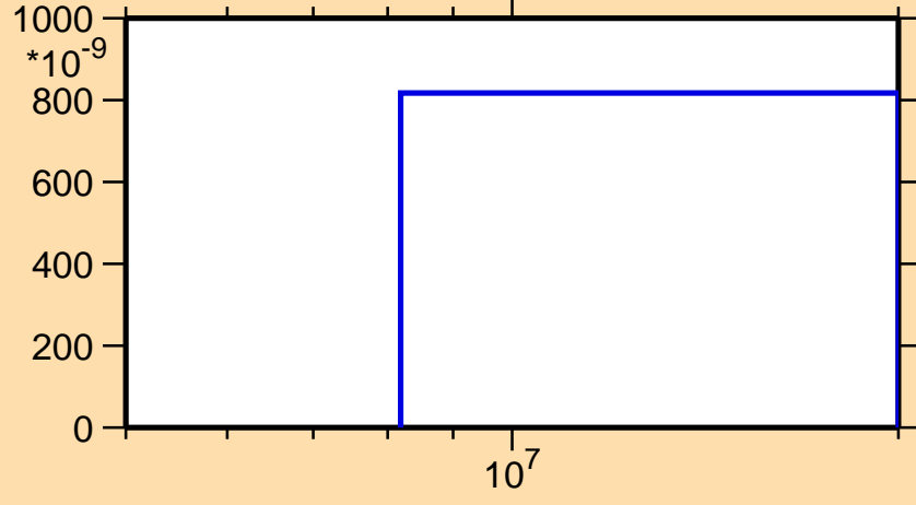
\sigma vs. E for ^{254}\text{Md}(n,nd)
