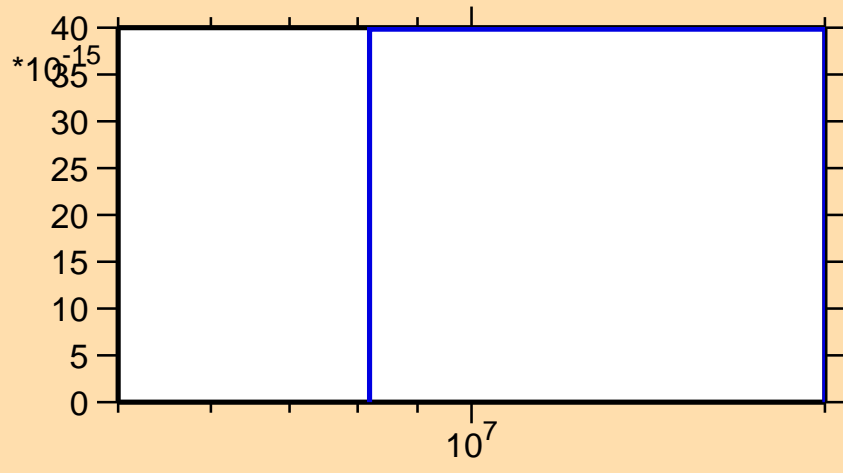
\sigma vs. E for ^{254}\text{Md}(\text{mt } 11)
