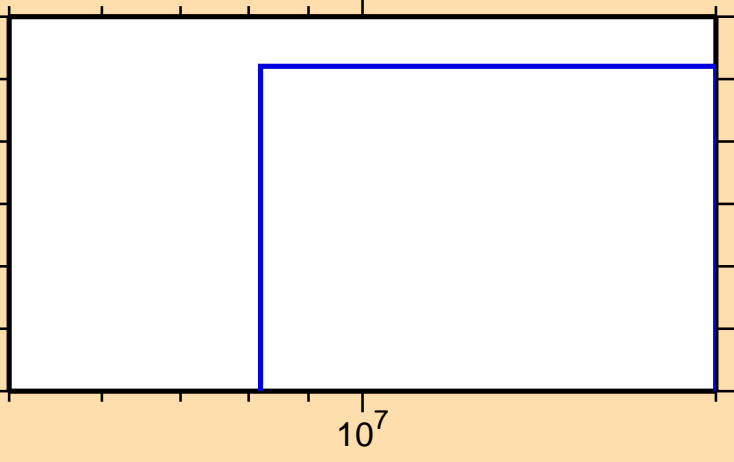
\sigma vs. E for ^{254}\text{Md}(n,\text{He3})
