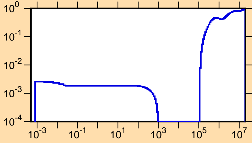
\mu vs. E for ^{255}\text{Md}(\text{mt251})
