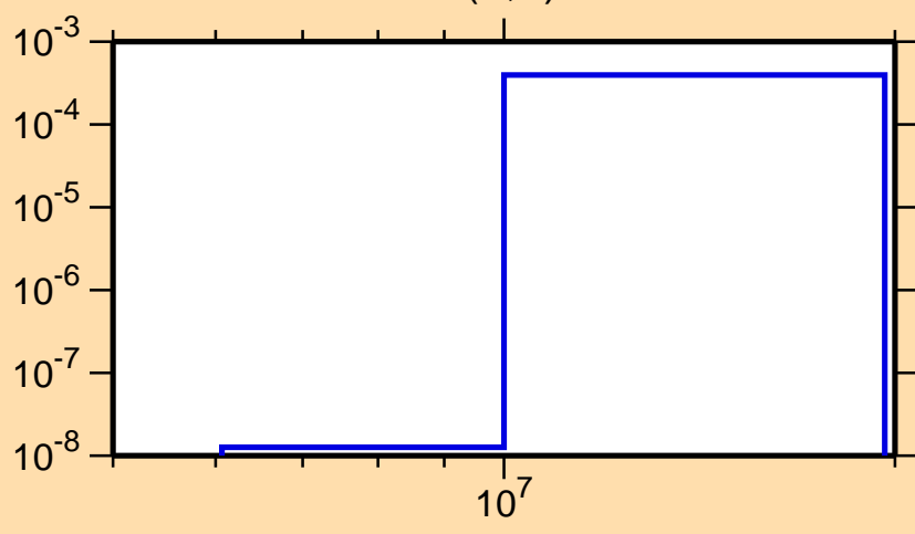
\sigma vs. E for ^{255}\text{Md}(n,d)
