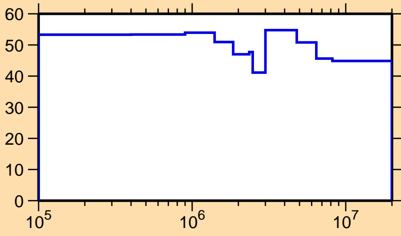
\Delta\sigma/\sigma vs. E for ^{255}\text{Md}(n,n_1)
