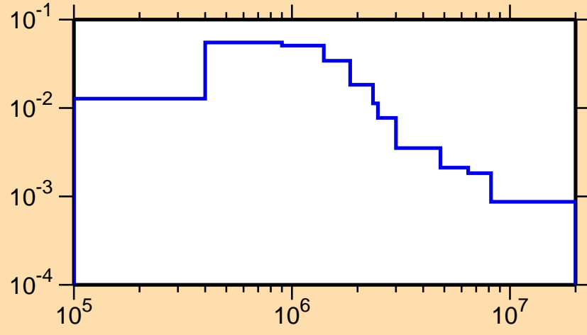
\sigma vs. E for ^{255}\text{Md}(n,n_2)
