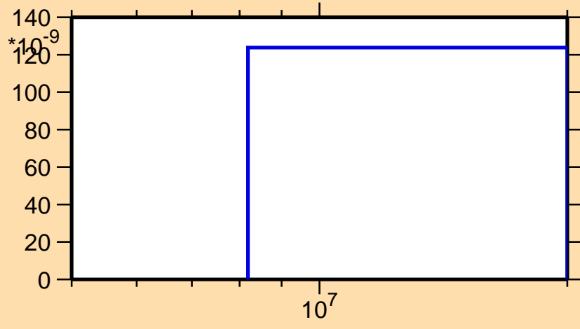
\sigma vs. E for ^{255}\text{Md}(n,nd)
