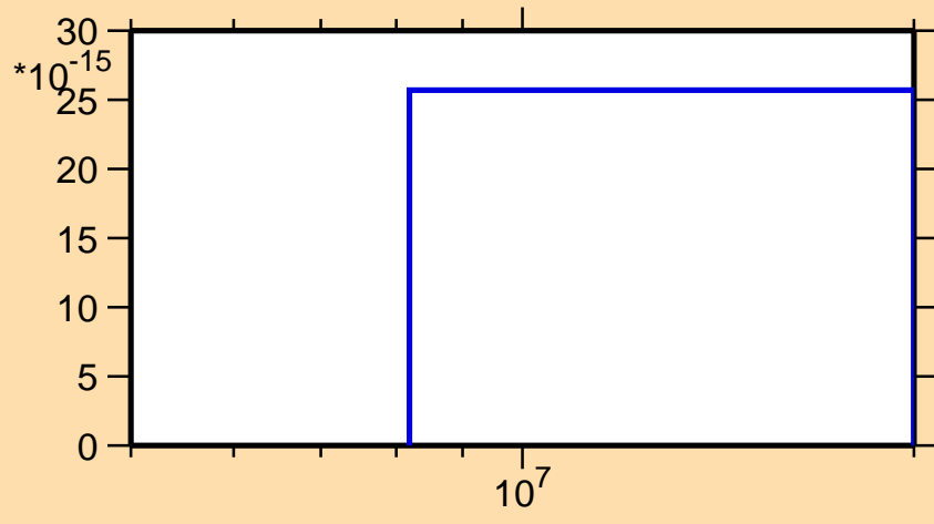
\sigma vs. E for ^{255}\text{Md} (mt 42)
