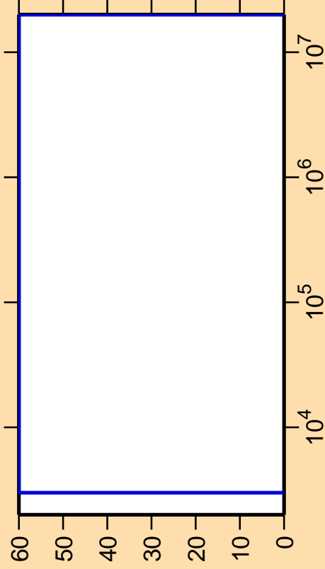
\Delta\sigma/\sigma vs. E for ^{255}\text{Md}(n,\gamma)
