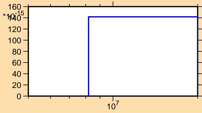
\sigma vs. E for ^{255}\text{Md}(\text{mt } 11)
