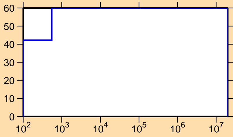
\Delta\sigma/\sigma vs. E for ^{255}\text{Md}(n,\gamma)
