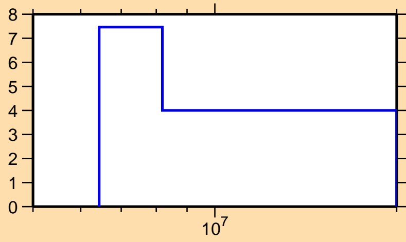
\Delta\sigma/\sigma vs. E for ^{255}\text{Md}(n,\text{tot.})
