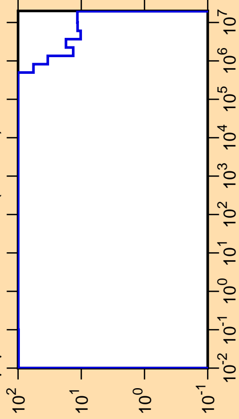
\Delta\mu/\mu vs. E for ^{256}\text{Md}(\text{mt251})
