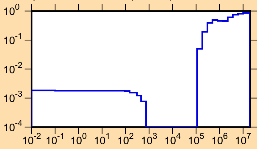
\mu vs. E for ^{256}\text{Md}(\text{mt251})
