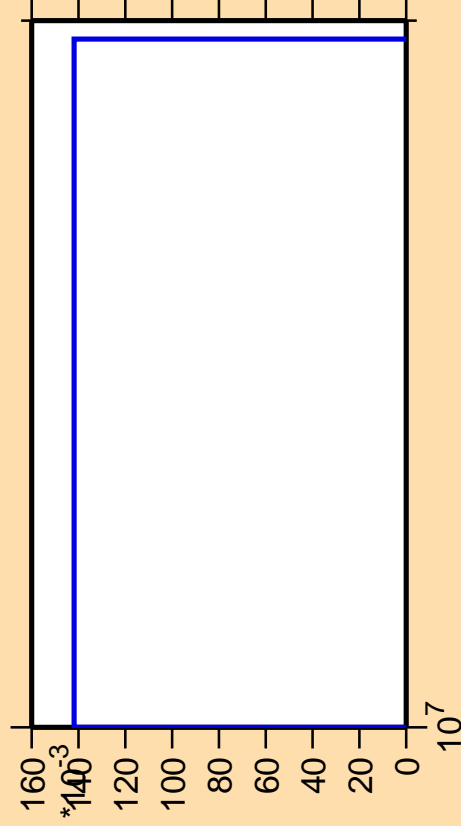
\Delta\sigma/\sigma vs. E for ^{256}\text{Md} (mt 11)
