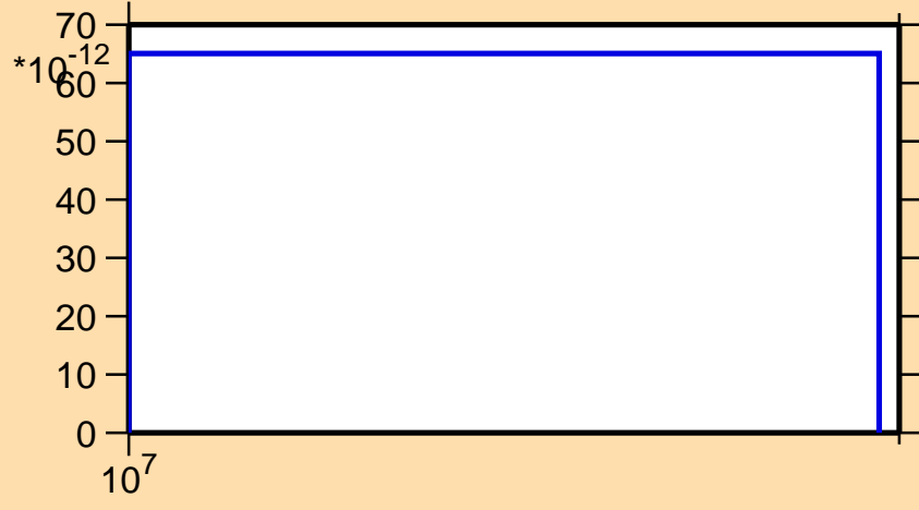
\sigma vs. E for ^{256}\text{Md}(n,\text{He3})
