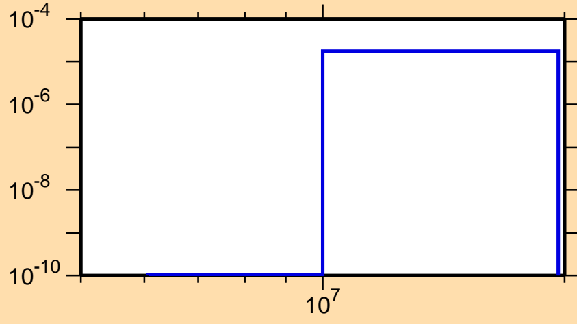
\sigma vs. E for ^{256}\text{Md}(\text{mt } 45)
