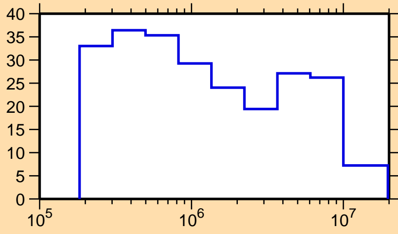
\Delta\sigma/\sigma vs. E for ^{256}\text{Md}(n,el.)
