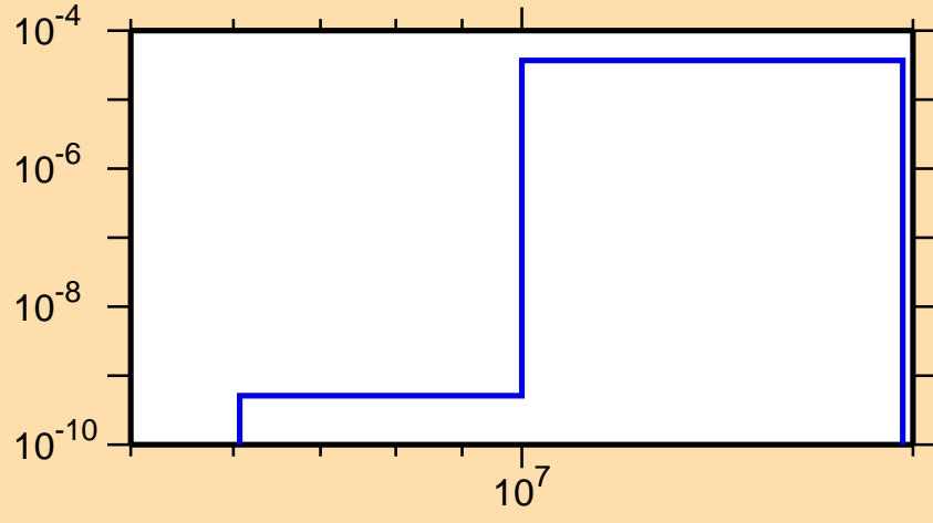
\sigma vs. E for ^{256}\text{Md}(\text{mt117})
