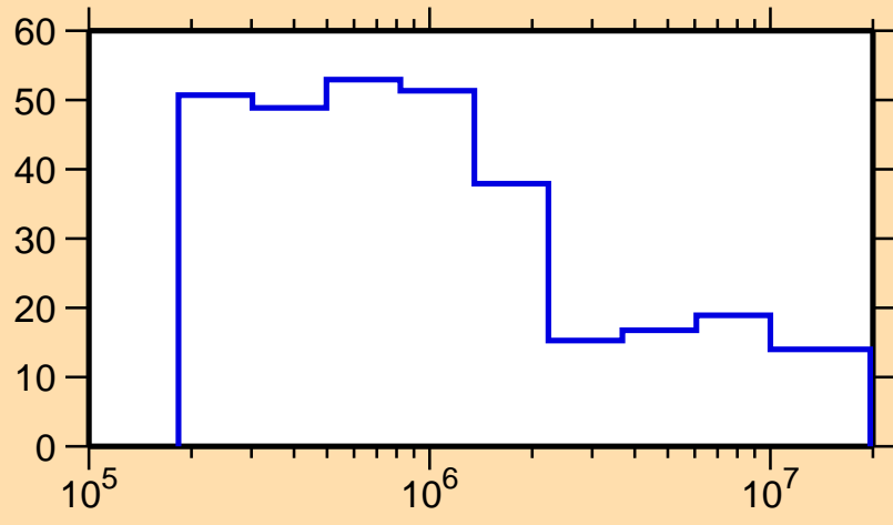
\Delta\sigma/\sigma vs. E for ^{256}\text{Md}(n,n\text{onel.})
