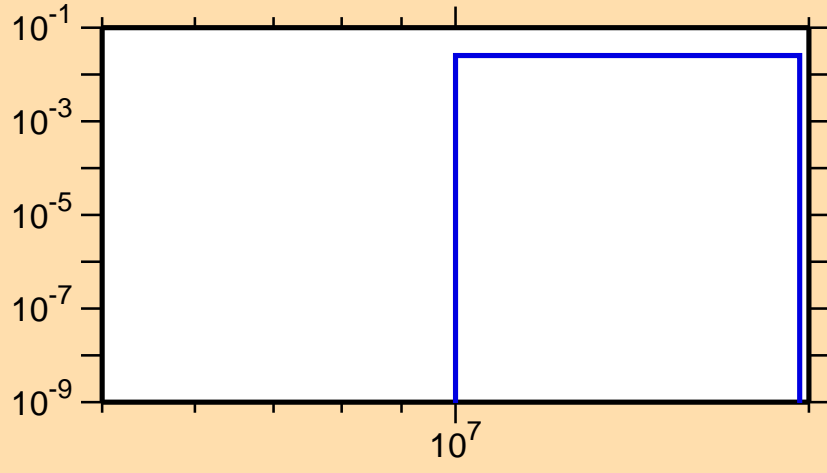
\sigma vs. E for ^{256}\text{Md}(n,3n\alpha)
