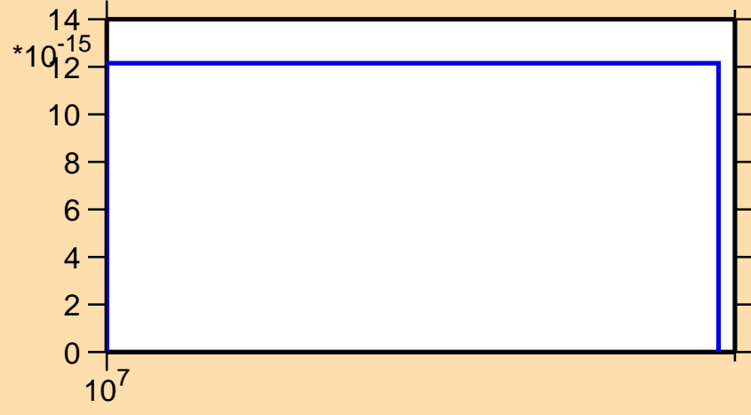
\sigma vs. E for ^{256}\text{Md} (mt 42)
