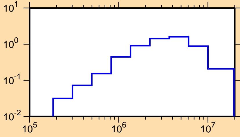
\sigma vs. E for ^{256}\text{Md}(n,n\text{cont.})
