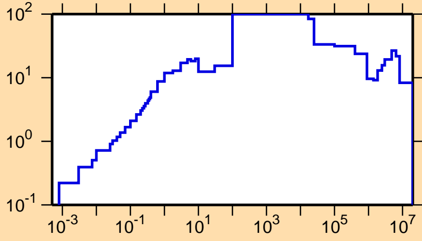
\Delta\sigma/\sigma vs. E for ^{256}\text{Md}(n,tot.)
