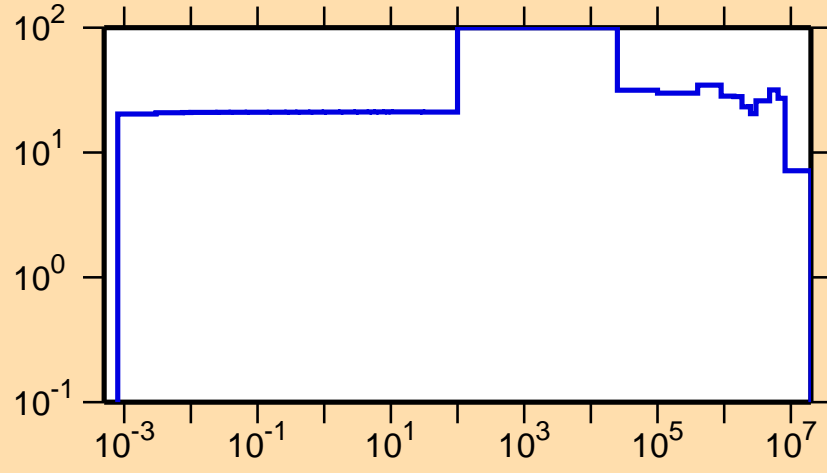
\Delta\sigma/\sigma vs. E for ^{256}\text{Md}(n,el.)
