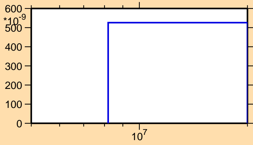
\sigma vs. E for ^{256}\text{Md}(n,nd)
