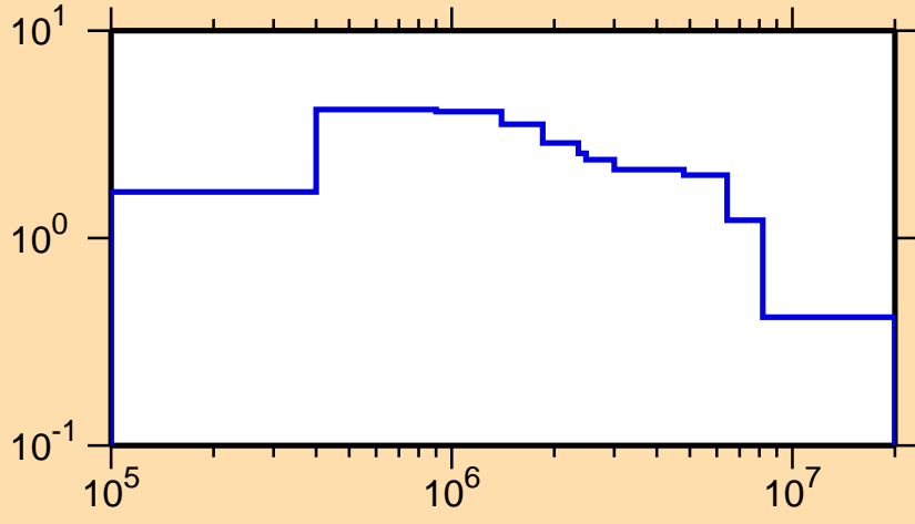
\sigma vs. E for ^{256}\text{Md}(n,\text{inel.})
