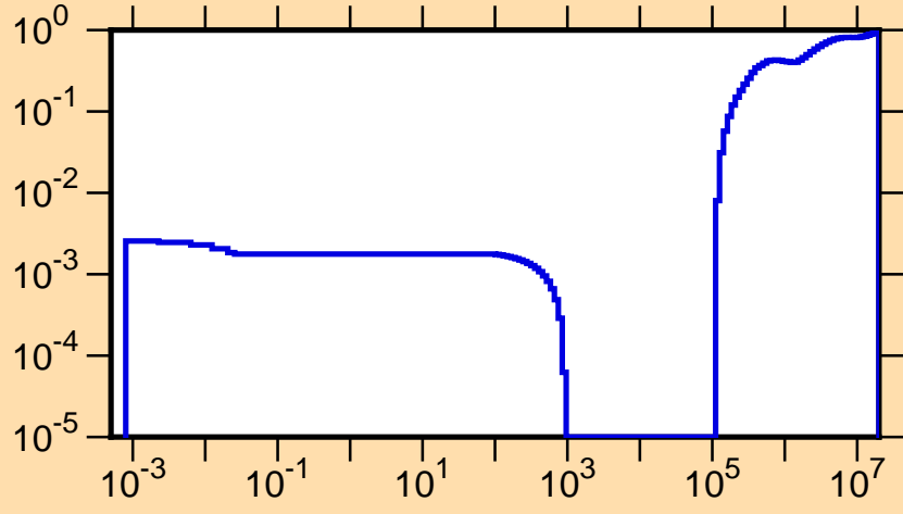
\mu vs. E for ^{257}\text{Md}(\text{mt251})
