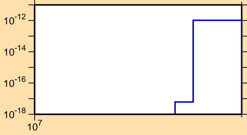
\sigma vs. E for ^{257}\text{Md} (mt 42)
