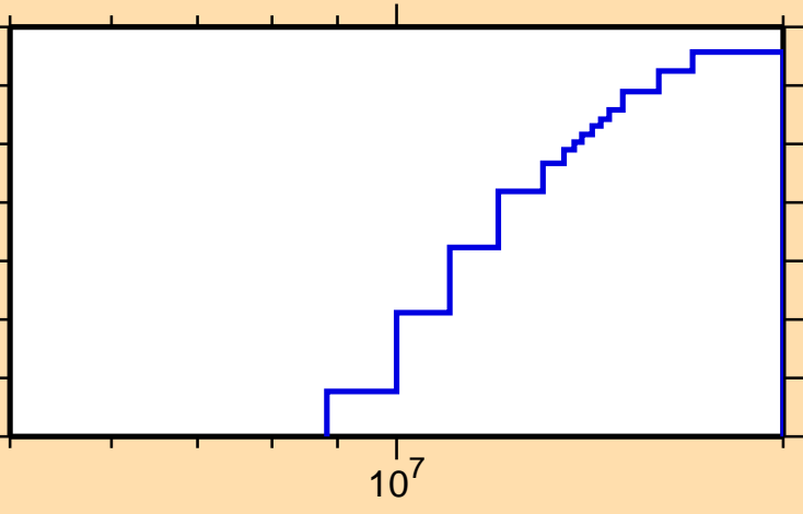
\sigma vs. E for ^{257}\text{Md}(\text{mt117})
