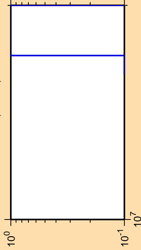
\Delta\sigma/\sigma vs. E for ^{257}\text{Md} (mt 42)
