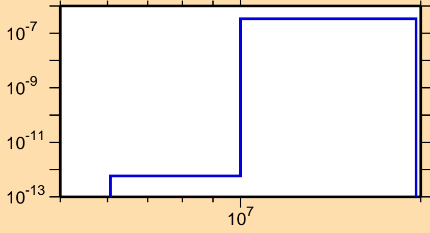
\sigma vs. E for ^{257}\text{Md}(\text{mt117})
