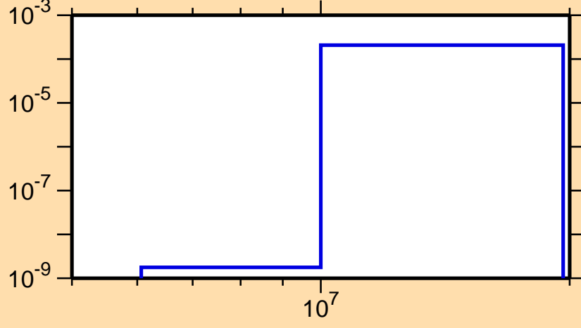
\sigma vs. E for ^{257}\text{Md}(n,np)
