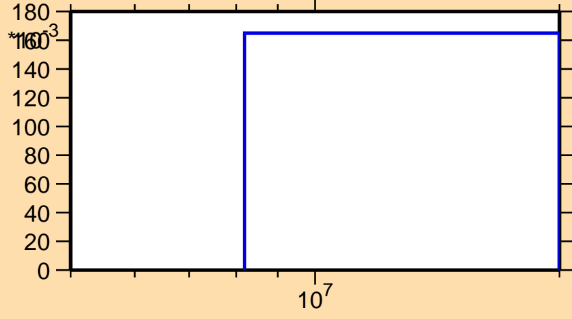
\sigma vs. E for ^{257}\text{Md}(n,3n)
