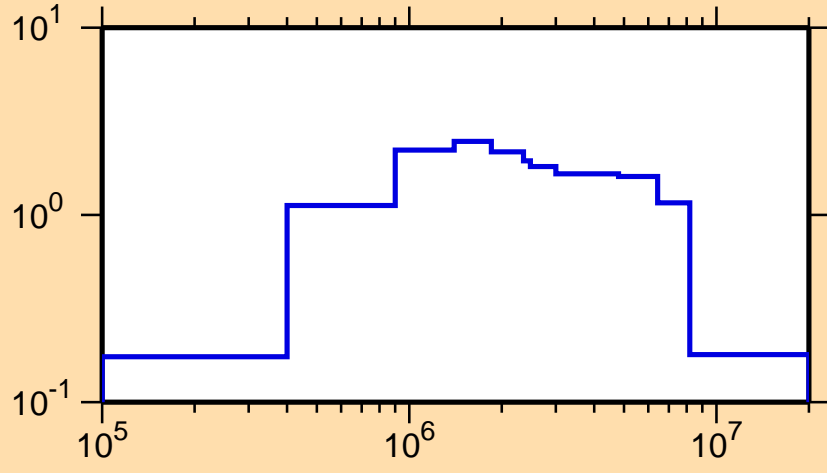
\sigma vs. E for ^{257}\text{Md}(n,n\text{cont.})
