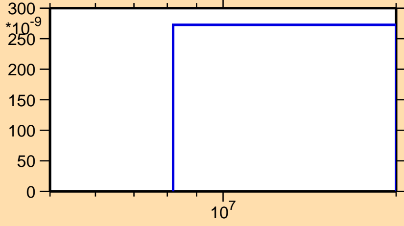
\sigma vs. E for ^{257}\text{Md}(\text{mt117})
