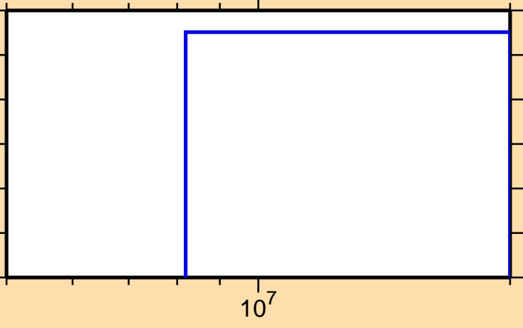
\sigma vs. E for ^{257}\text{Md}(n,nt)
