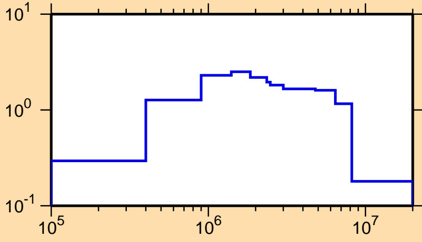
\sigma vs. E for ^{257}\text{Md}(n,\text{inel.})
