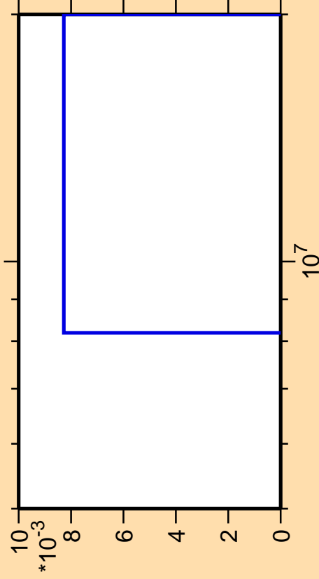
\Delta\sigma/\sigma vs. E for ^{257}\text{Md} (mt 42)
