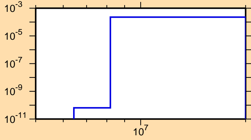
\sigma vs. E for ^{257}\text{Md}(n,d)
