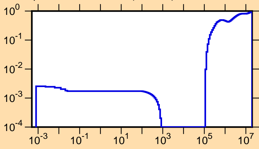
\mu vs. E for ^{258}\text{Md}(\text{mt251})
